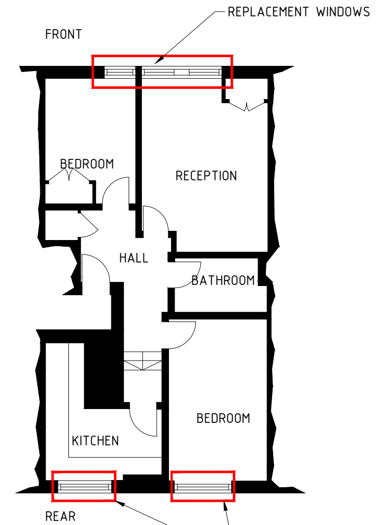
PLAN - PROPOSED
