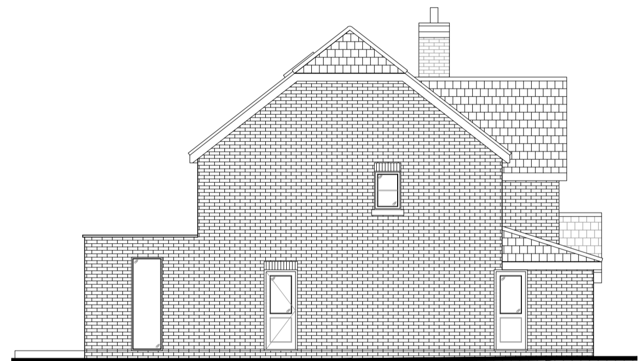
4 PROPOSED SIDE ELEVATION 1:100
