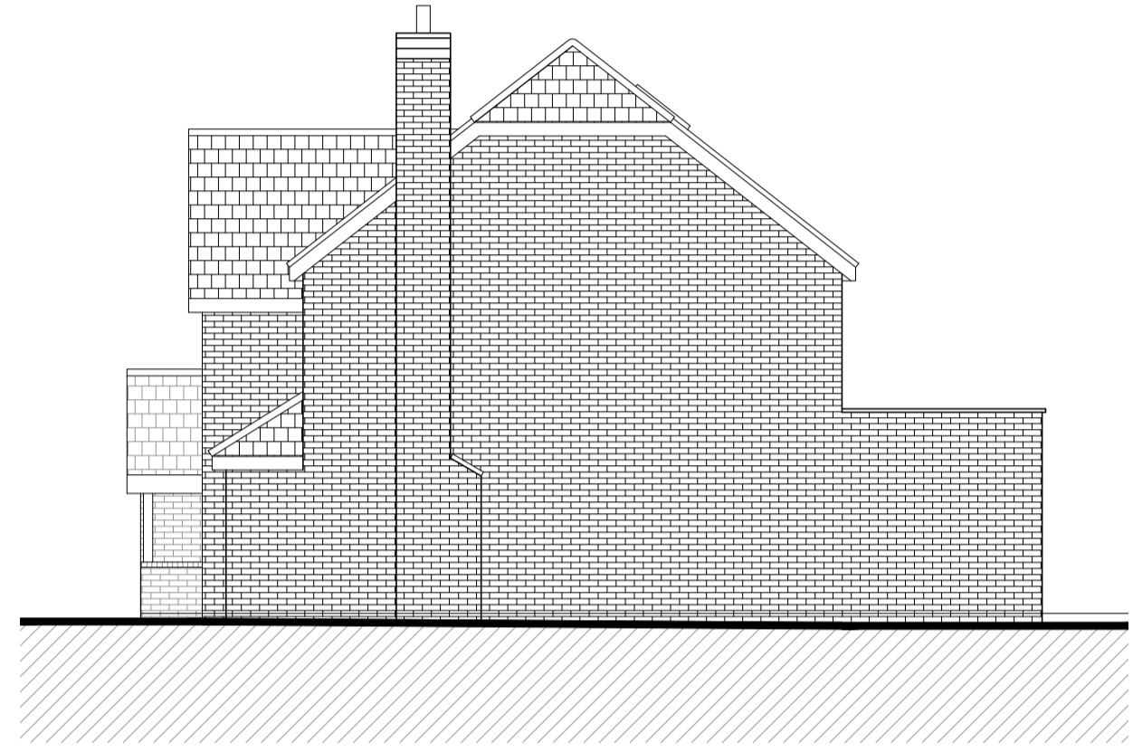
2 PROPOSED SIDE ELEVATION 1:100
