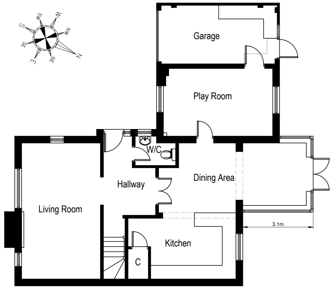
Ground floor plan @ 1:100 scale
