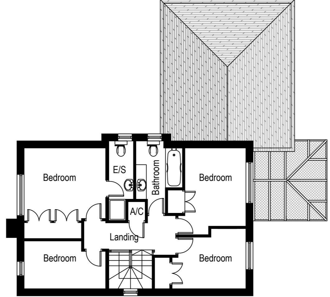
First floor plan @ 1:100 scale
