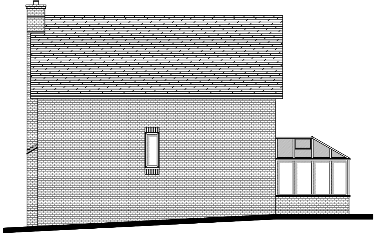
East elevation @ 1:100 scale
