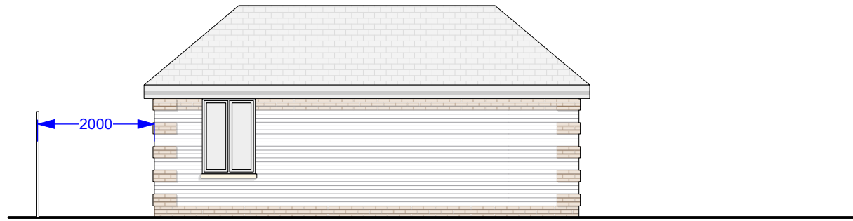
2 REAR ELEVATION_EAST SK-52 PROPOSED
