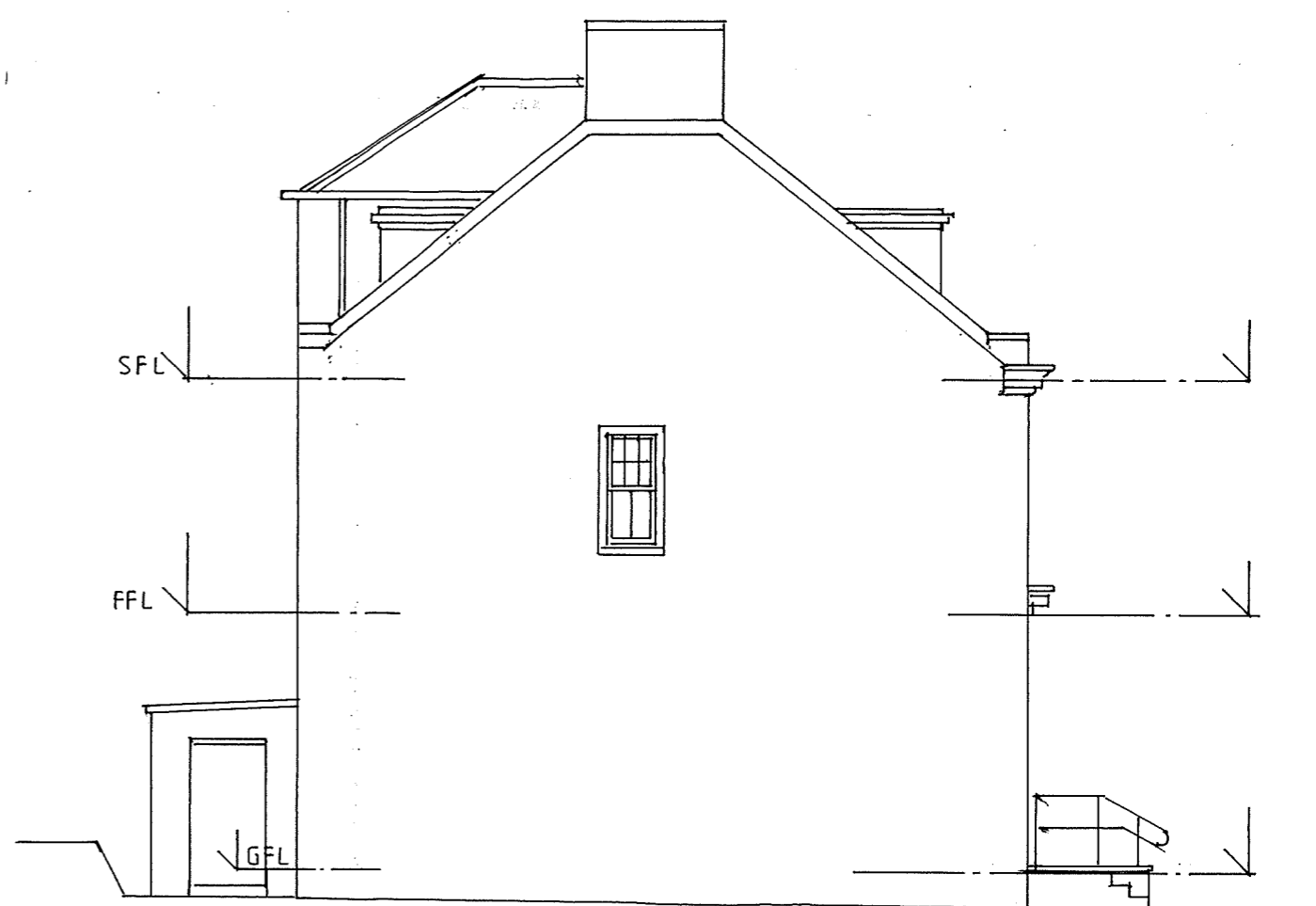
WEST ELEVATION
