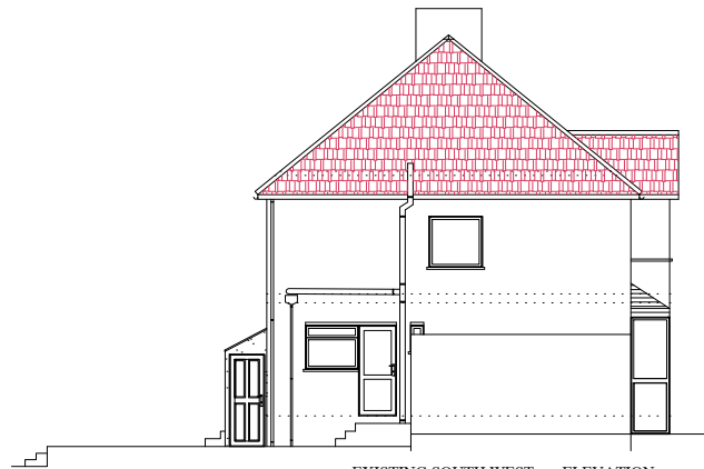
EXISTING SOUTH WEST ELEVATION
