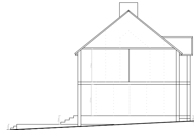
EXISTING SECTION A-A
