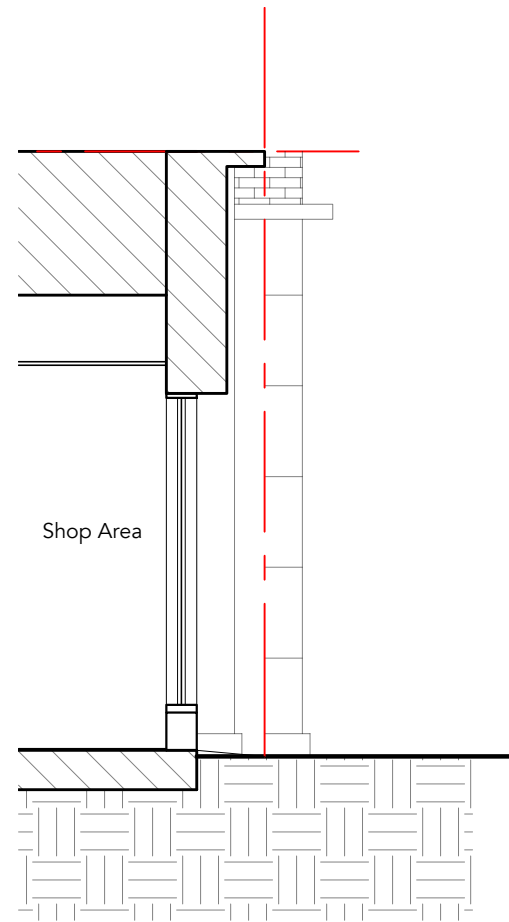
EXISTING PART SECTION
