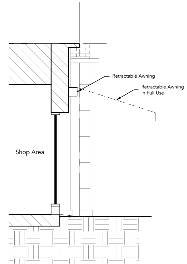
PROPOSED PART SECTION
