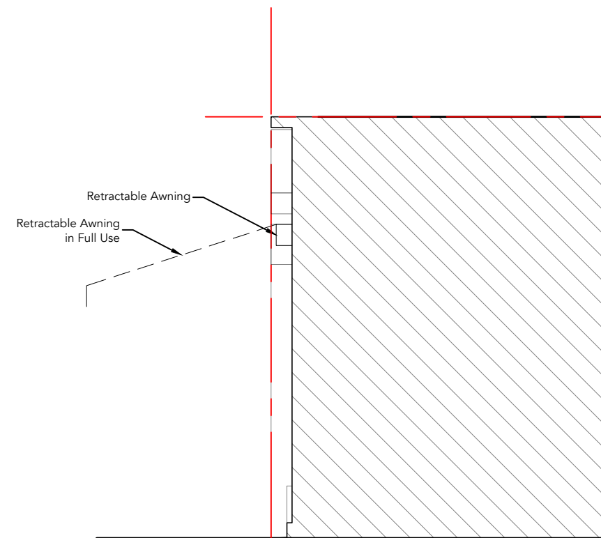
PROPOSED PART ELEVATION - SOUTH
