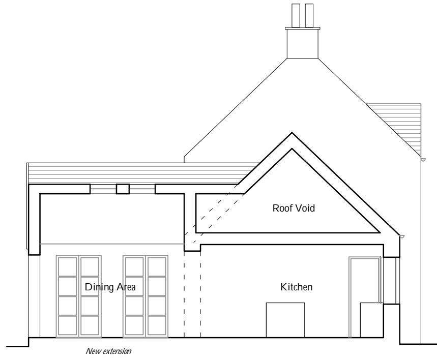
1 Section C-C As Proposed
