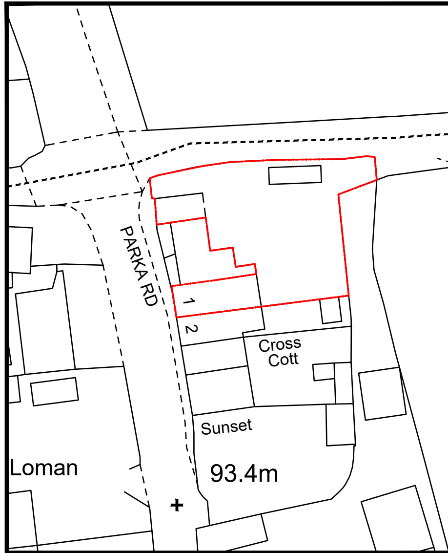
Block plan 1:500
