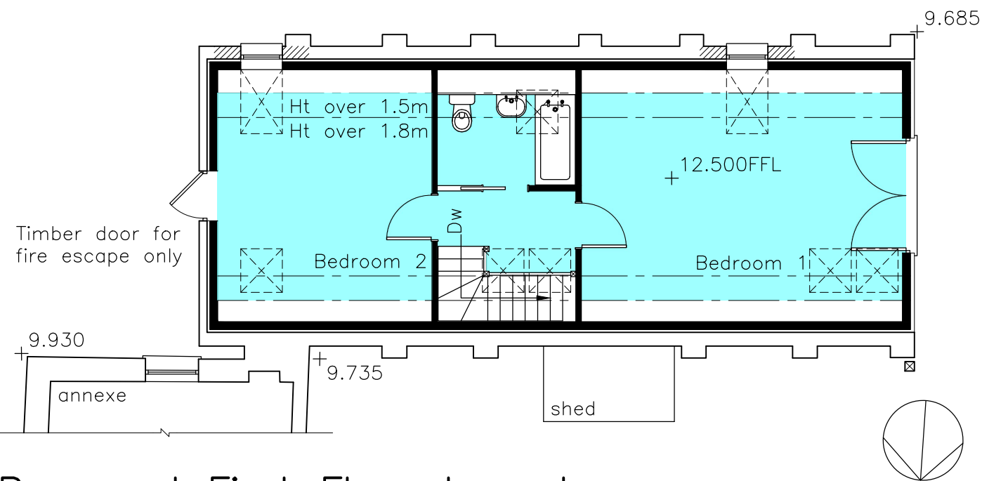
Proposed First Floor Layout 1:100
