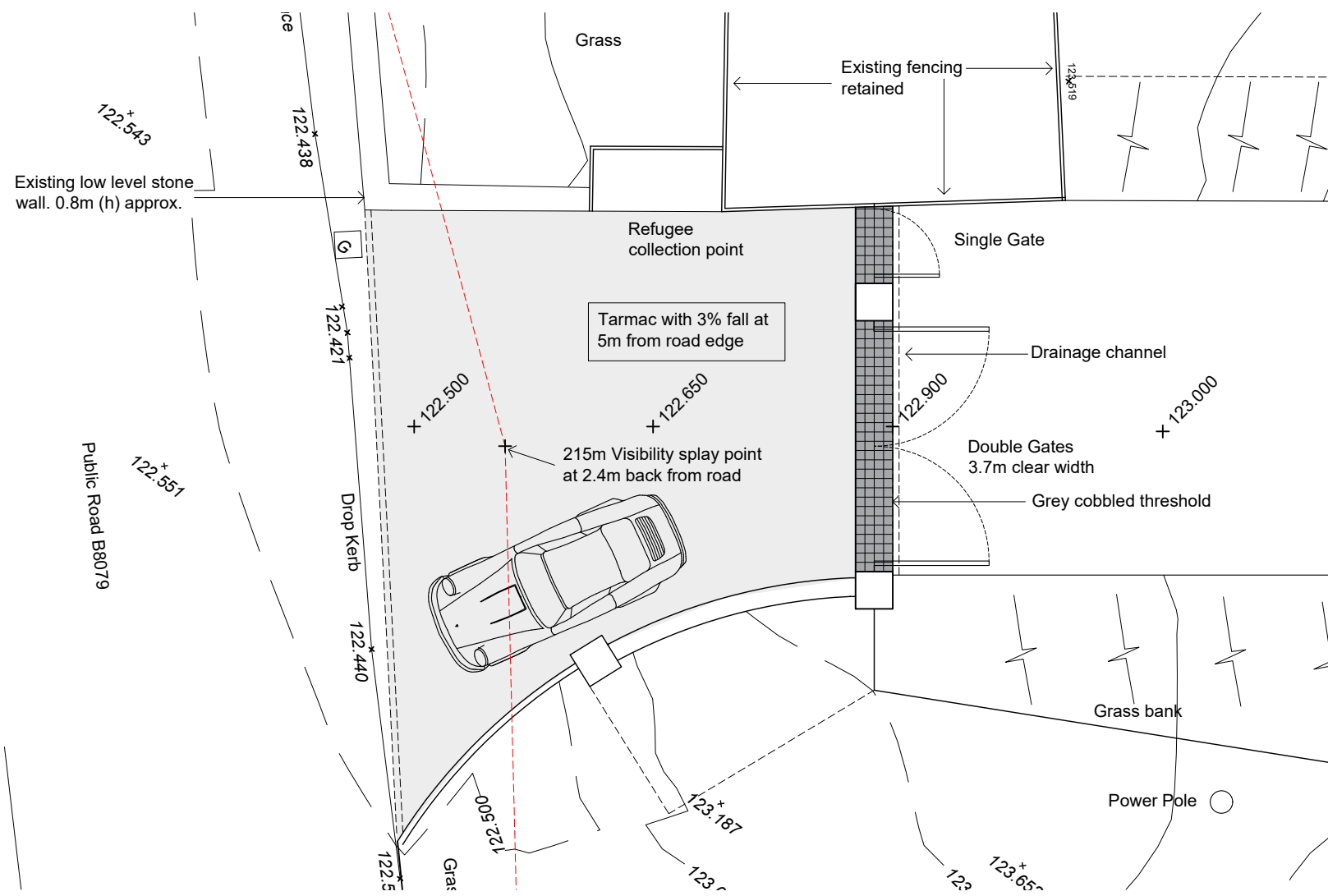
Plan of Junction Access
