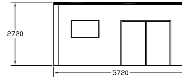
SOUTH FACING ELEVATION
