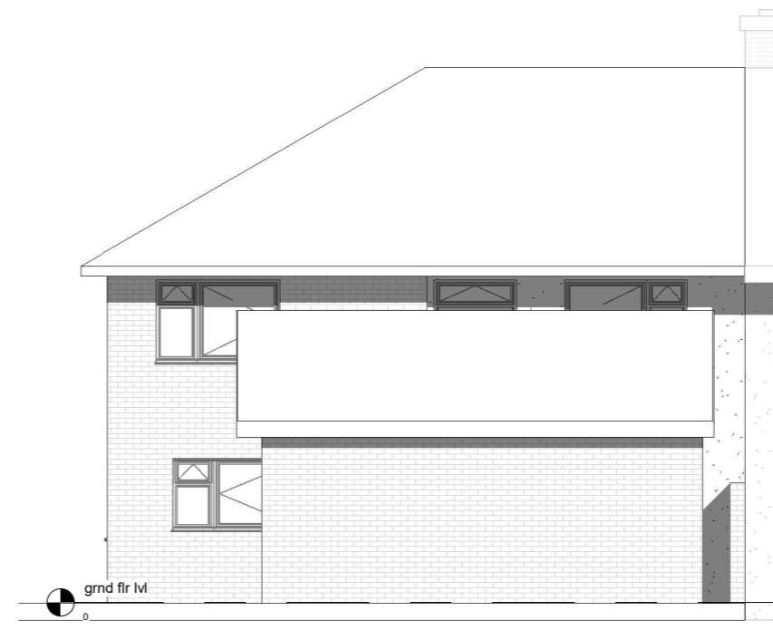
Existing Elevation-Front EAST
