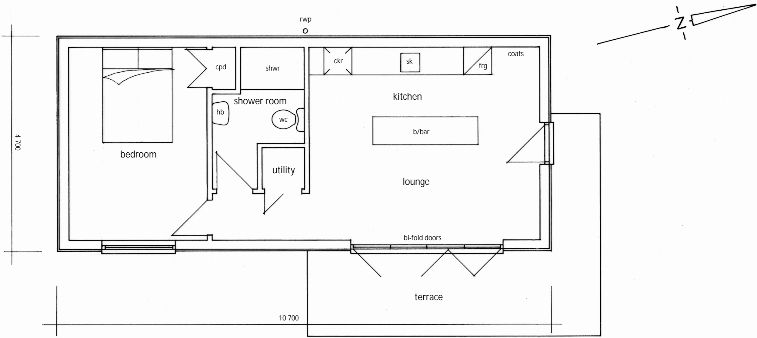
Floor Plan
