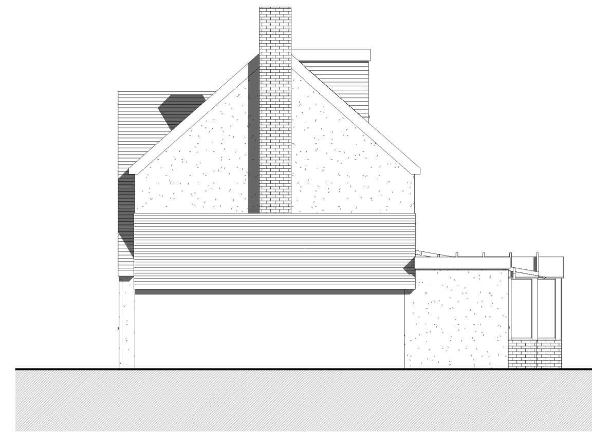
E Existing East Elevation 1:100
