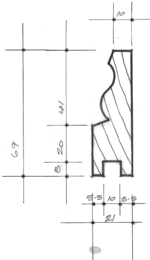
69 DEEP OGEE SKIRTING CAP PIECE FULL SIZE
