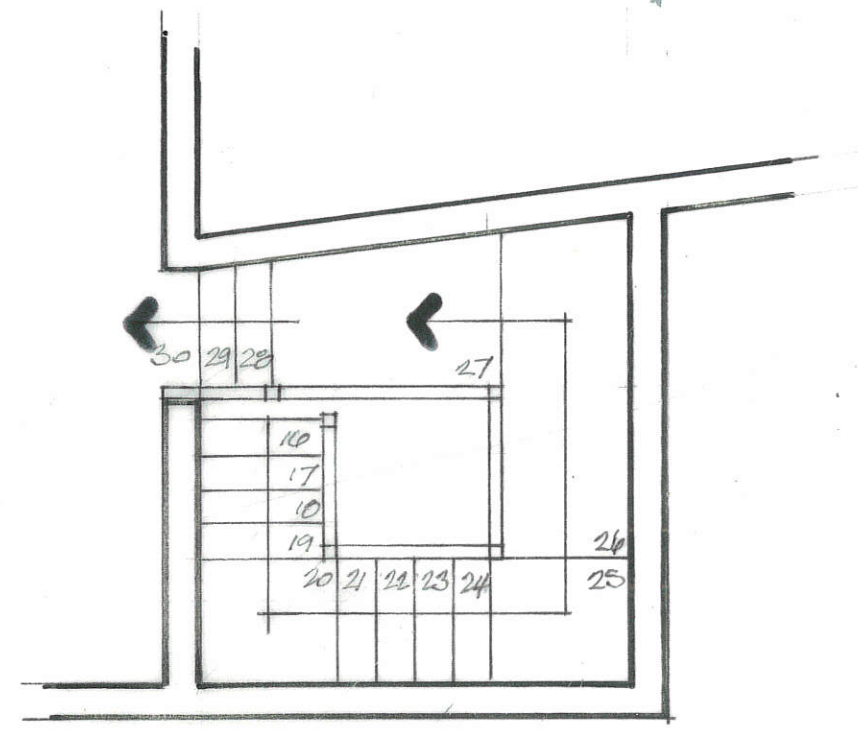
1ST FLOOR PLAN 1:50
