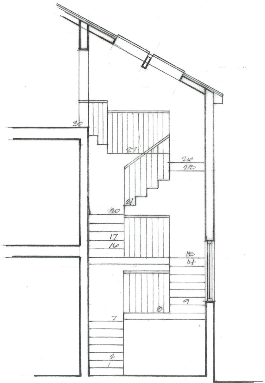
SECTION 1:50
