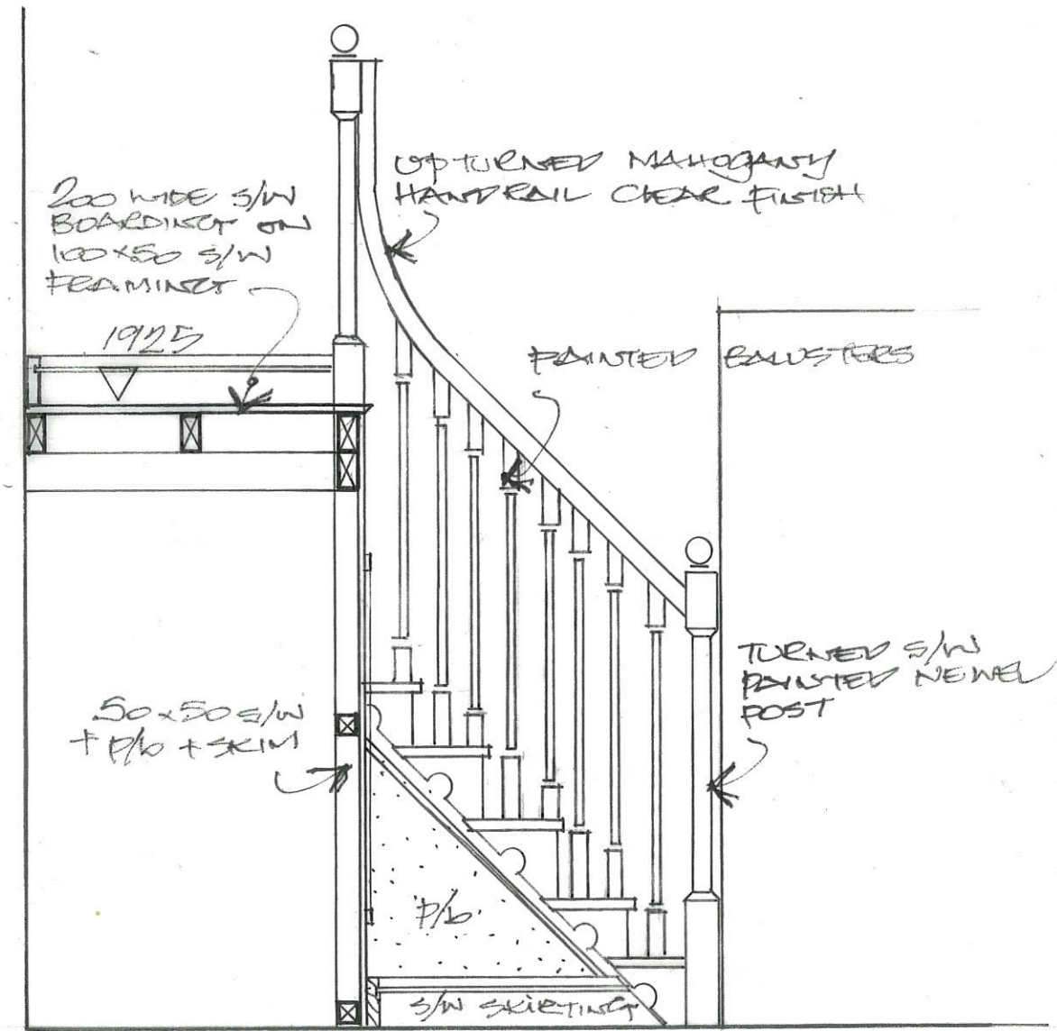
SECTION/ ELEVATION C-C.
