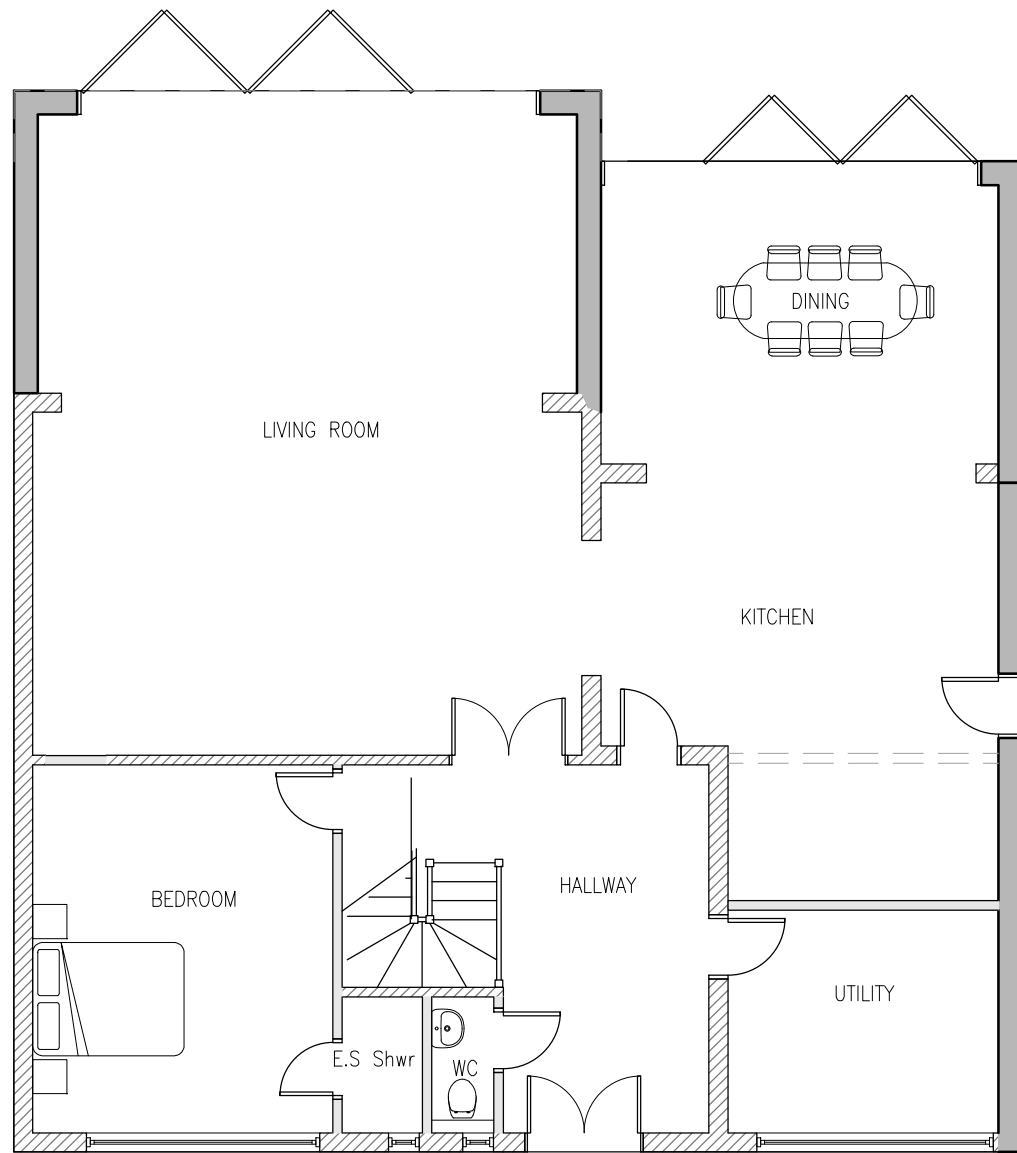
Existing GROUND FLOOR PLAN 181 sq.m
