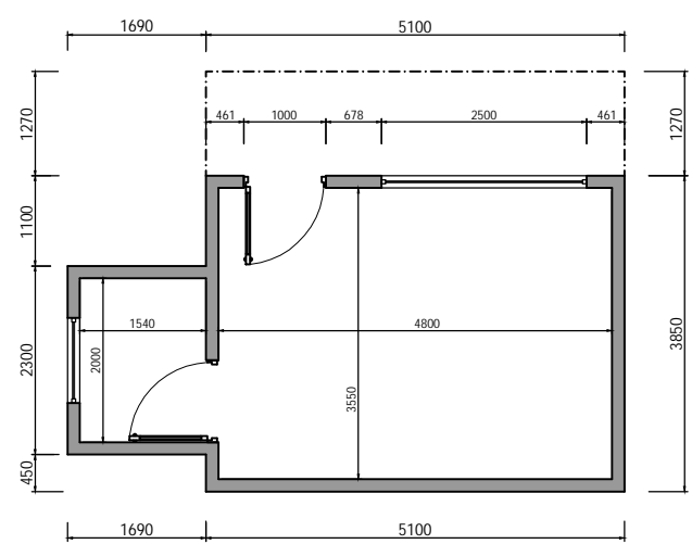
⊖ Floor plan 1:50@A3
