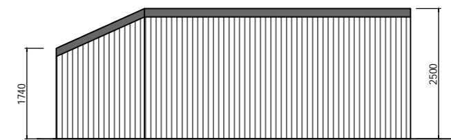
⊖ Rear elevation
