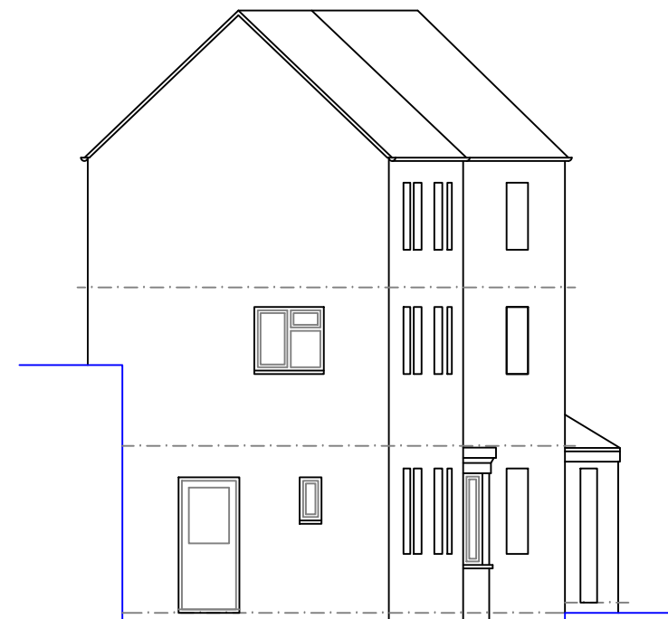
NORTH ELEVATION
