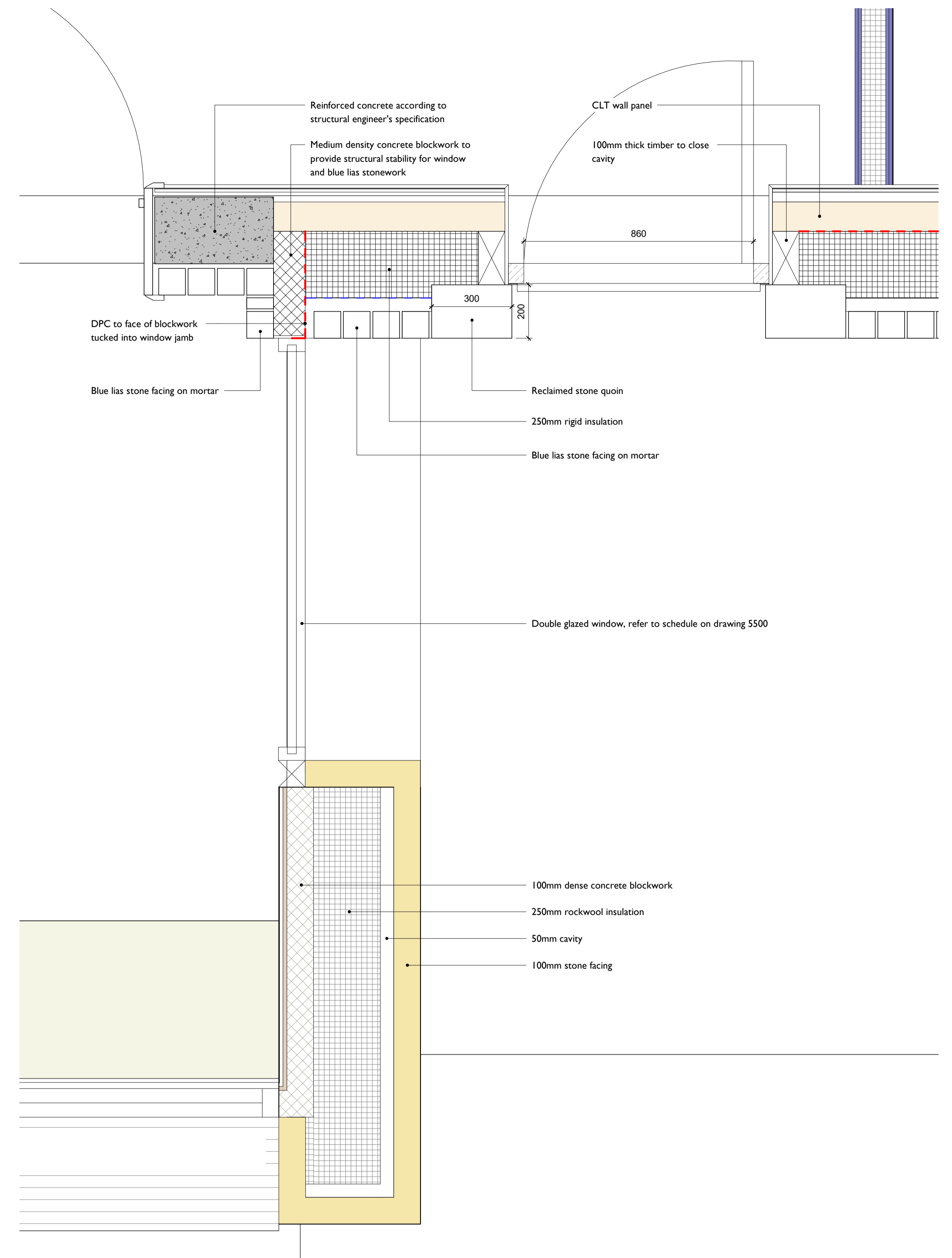
End bay window corner detail 1:10
