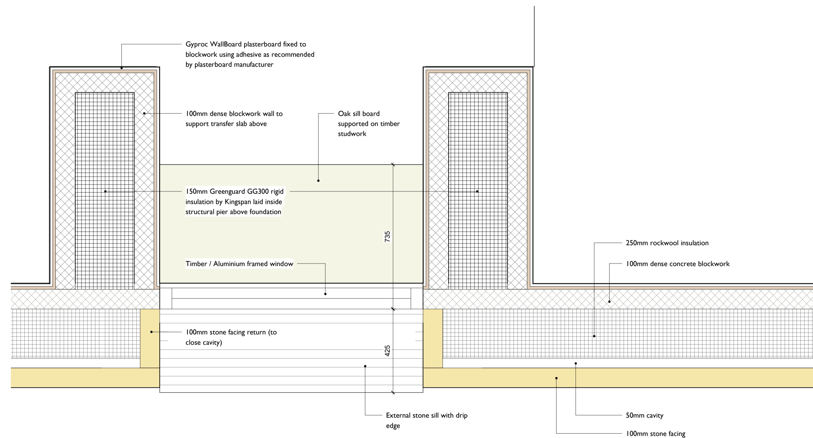
GF Bay Window Detail 1:10
