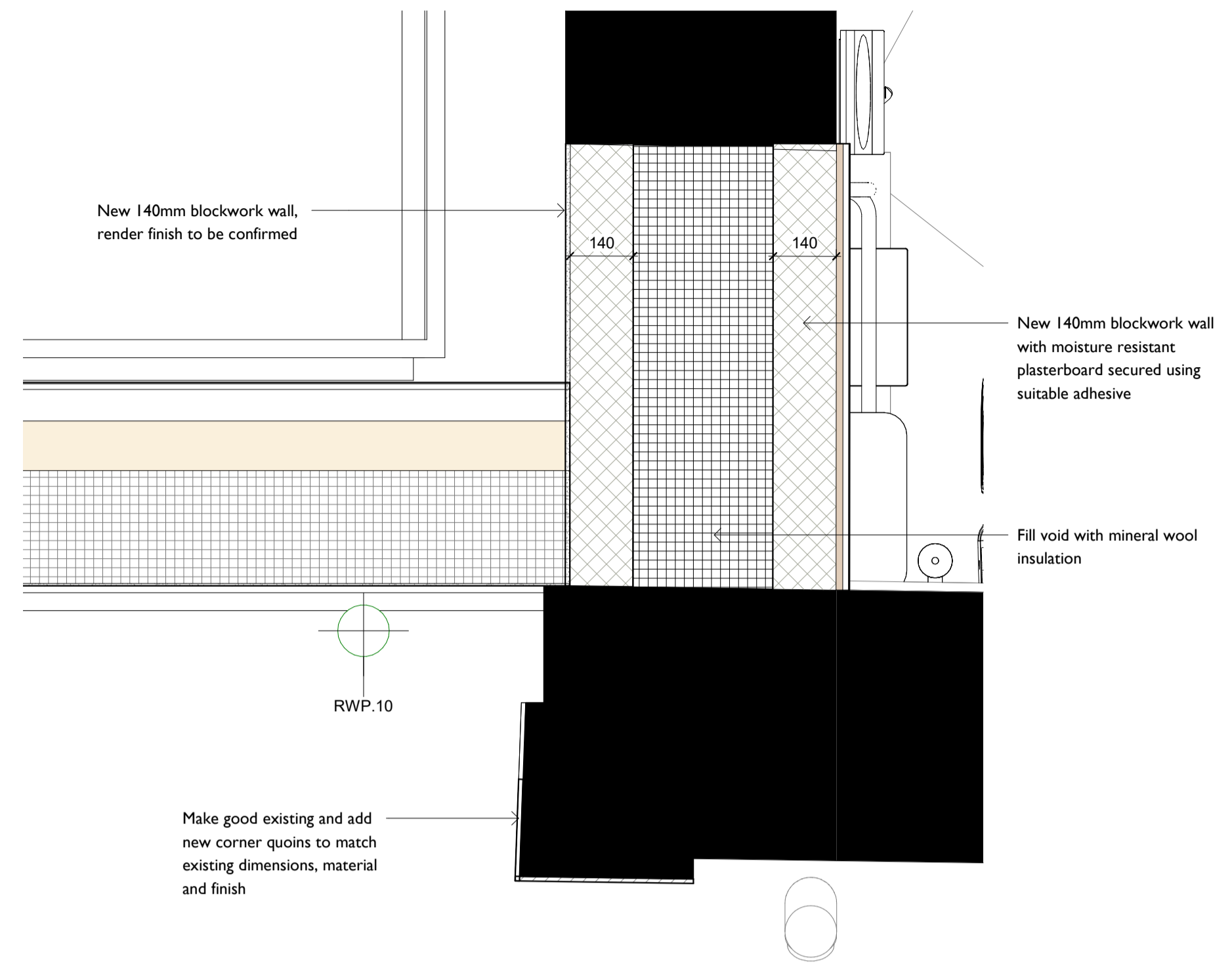
New to existing wall abutment detail 1:10
