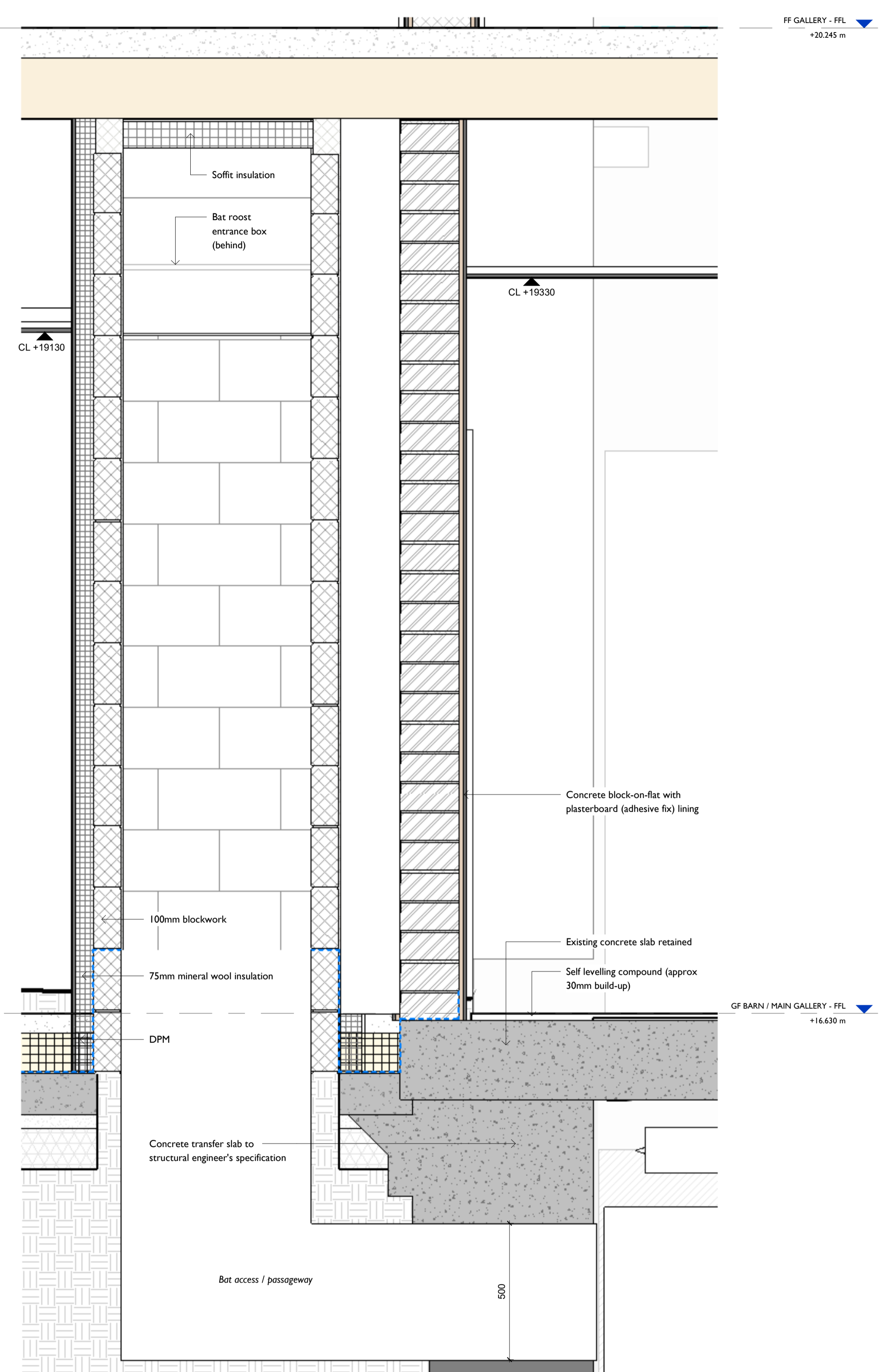
Bat Shaft Detail 2 1 : 10
