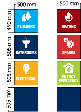
Sign 7 - 8no. Externally applied digitally printed vinyl. Cap Height = 65mm
