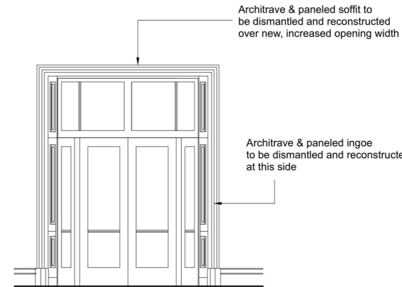
PROPOSED INTERNAL ELEVATION 1:50 @ A3
