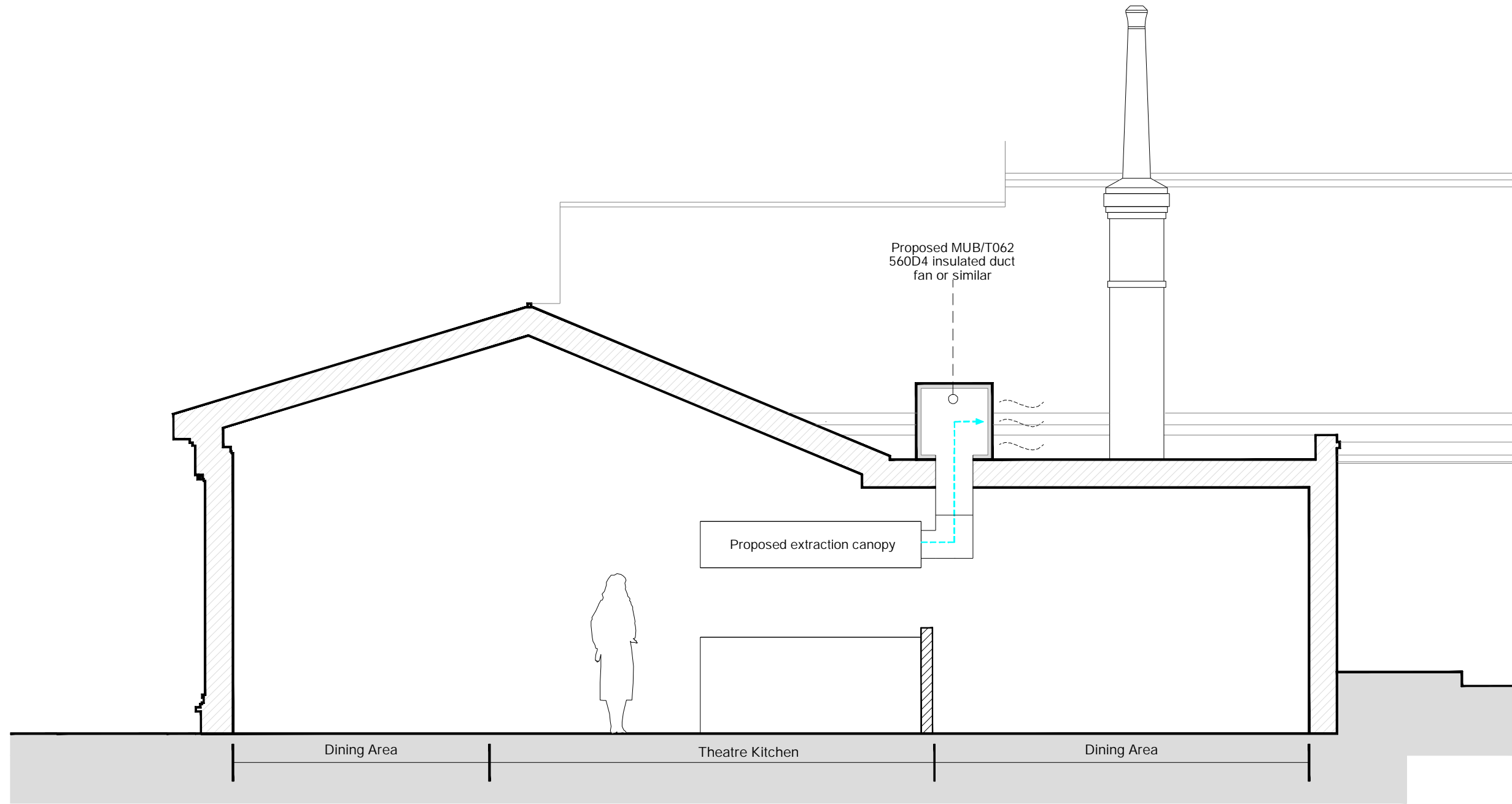
Illustrative Proposed Section 1:50 @ A3
