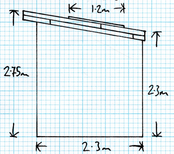
side elevation 2
