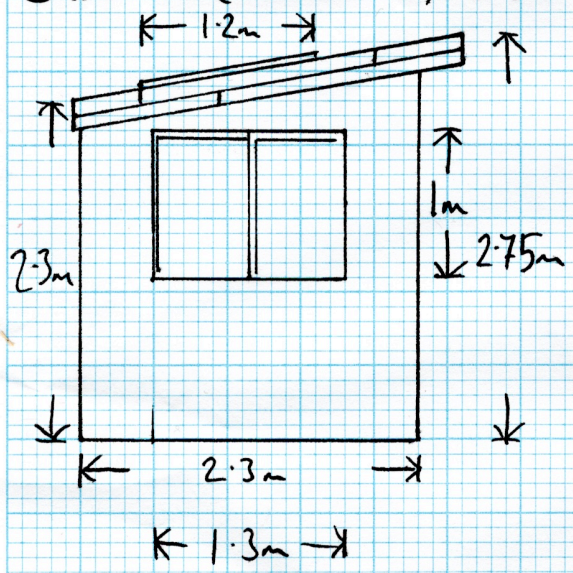
rear elevation 1:50
