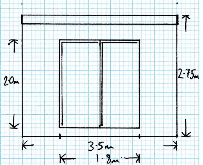
Front elevation 1:50
