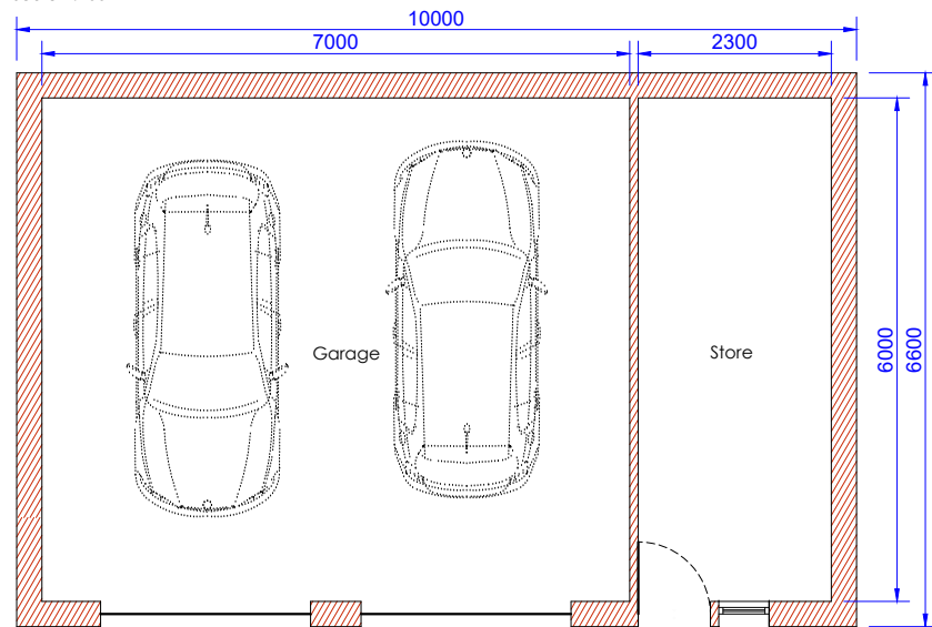
Proposed Ground Floor scale 1:100
