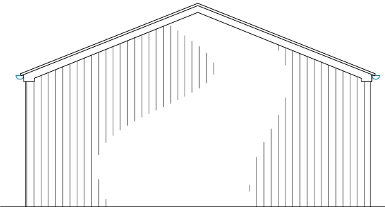
South scale 1:100
