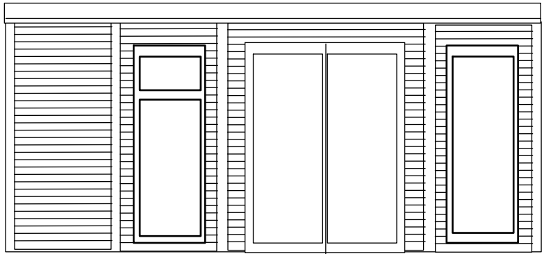
Front Elevation Painted Timber Clad Finish (South Facing)
