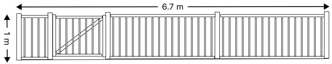
Front Elevation Treated Timber Finish (West Facing)
