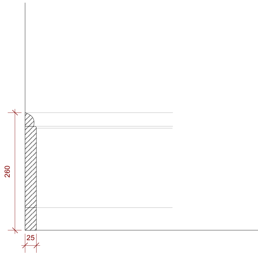
Existing Skirting Type 02 to be match where indicated
