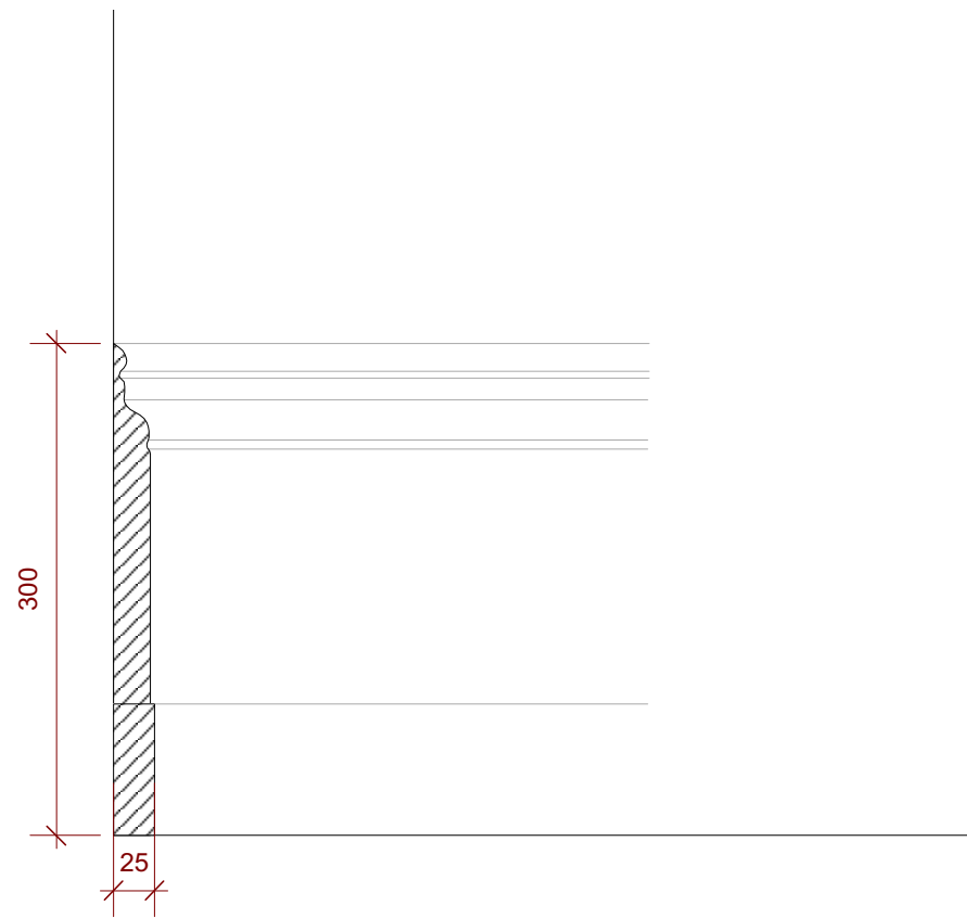
Existing Skirting Type 01 to be match where indicated
