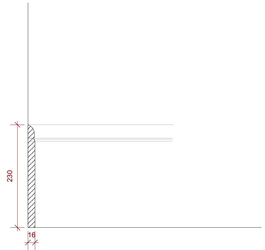
Existing Skirting Type 03 to be reused/replaced
