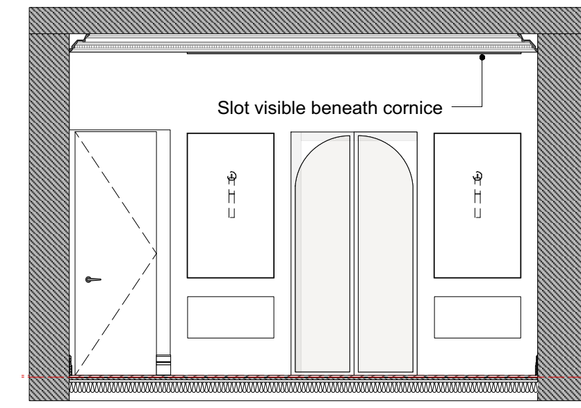
Air Conditioning Section Master Suite Elevation 1:50
