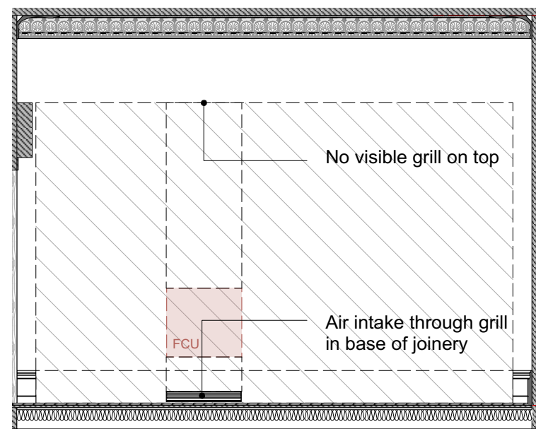
Air Conditioning Elevation Living Room Joinery Elevation 1:50
