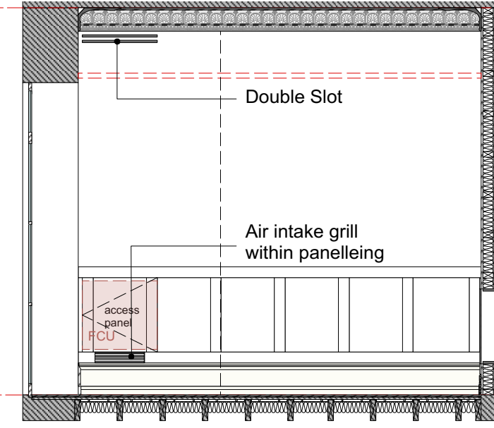
Air Conditioning Elevation Guest Bedroom Elevation 1:50
