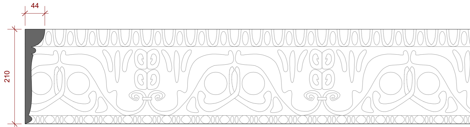
Existing Cornice Zones 3 and 4 To be matched as existing with scribed mitred edges
