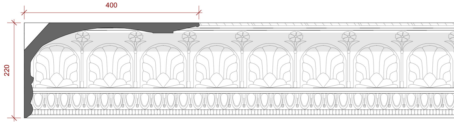
Existing Cornice Zones 1 and 2 To be matched as existing with scribed mitred edges
