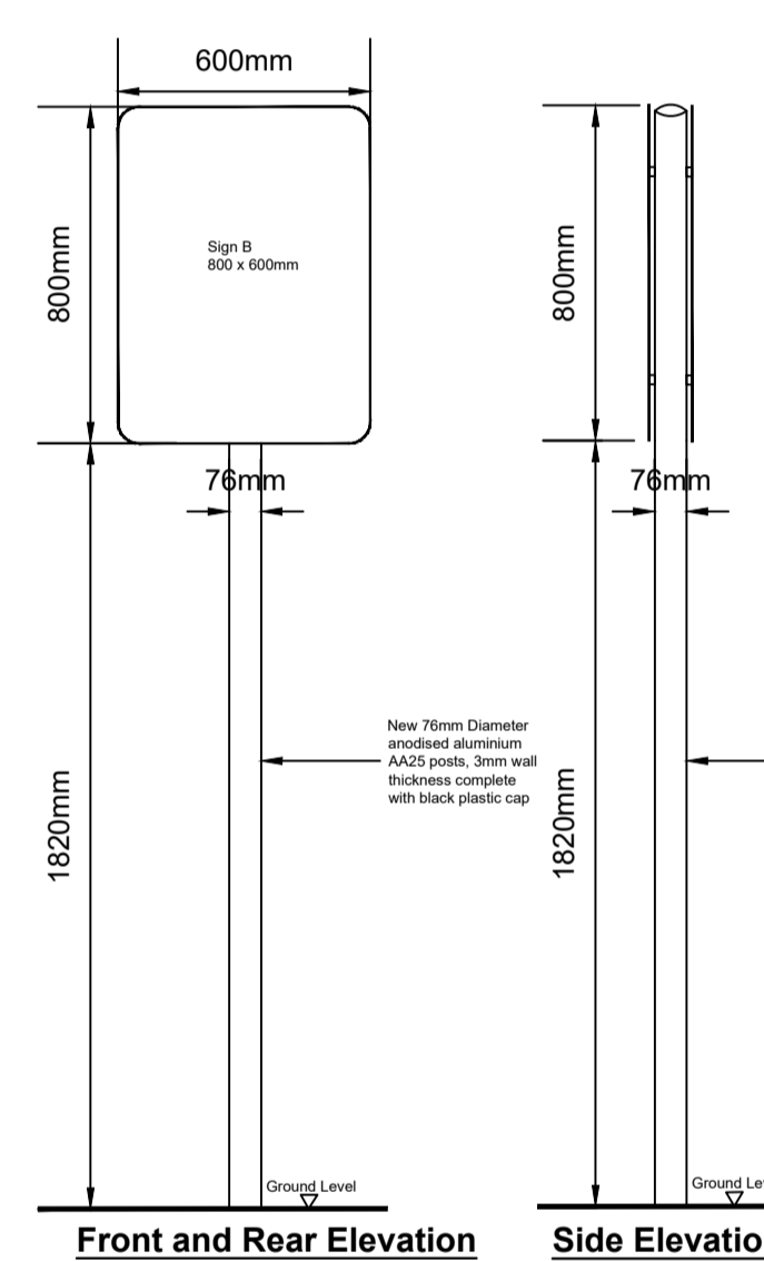
Sign #12 and #13 Double Sided Mounted on new posts 1820mm from ground level
