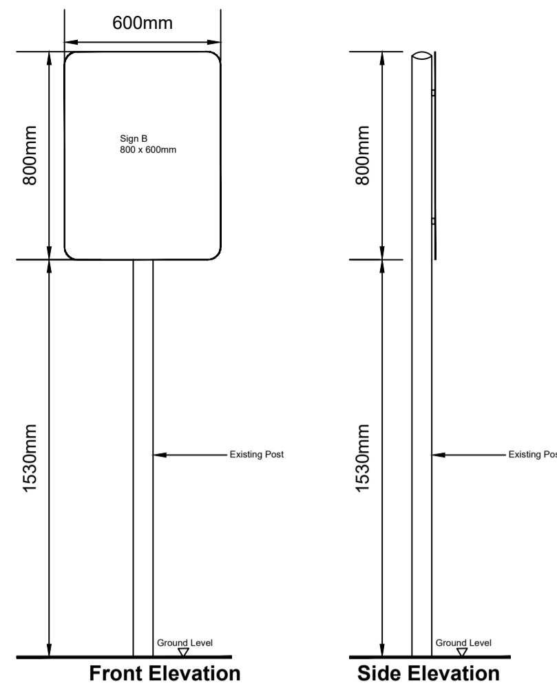
Sign #3 and #4 Mounted on old existing posts 1530mm from ground level
