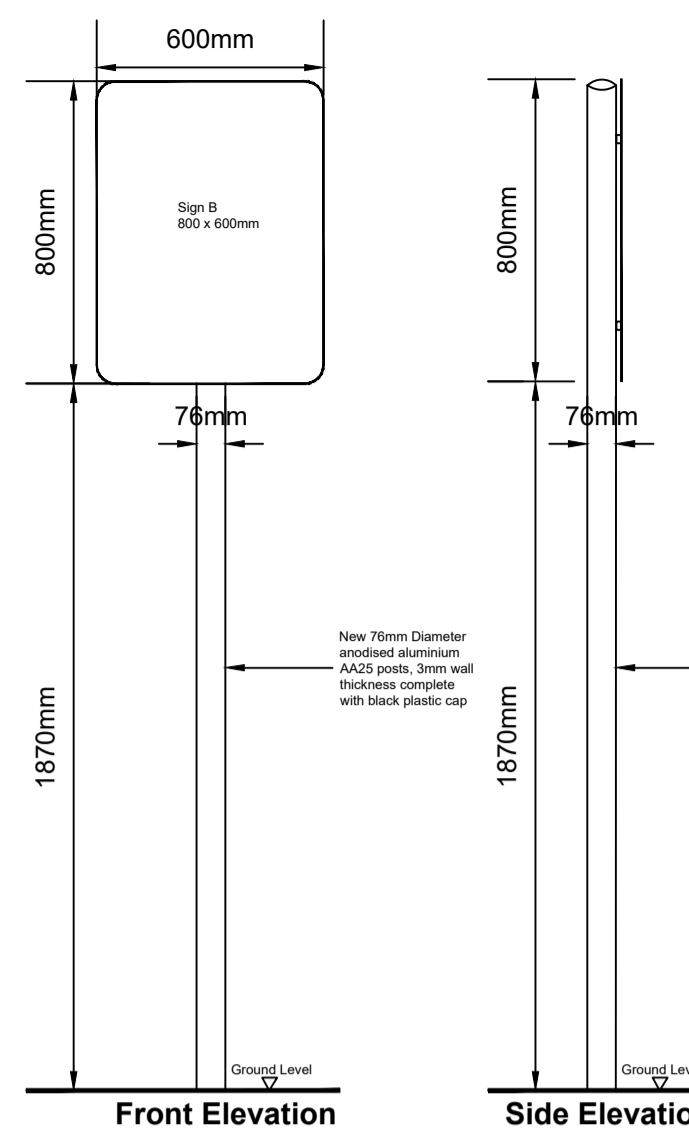
Sign #5 and #6 Mounted on new posts 1870mm from ground level
