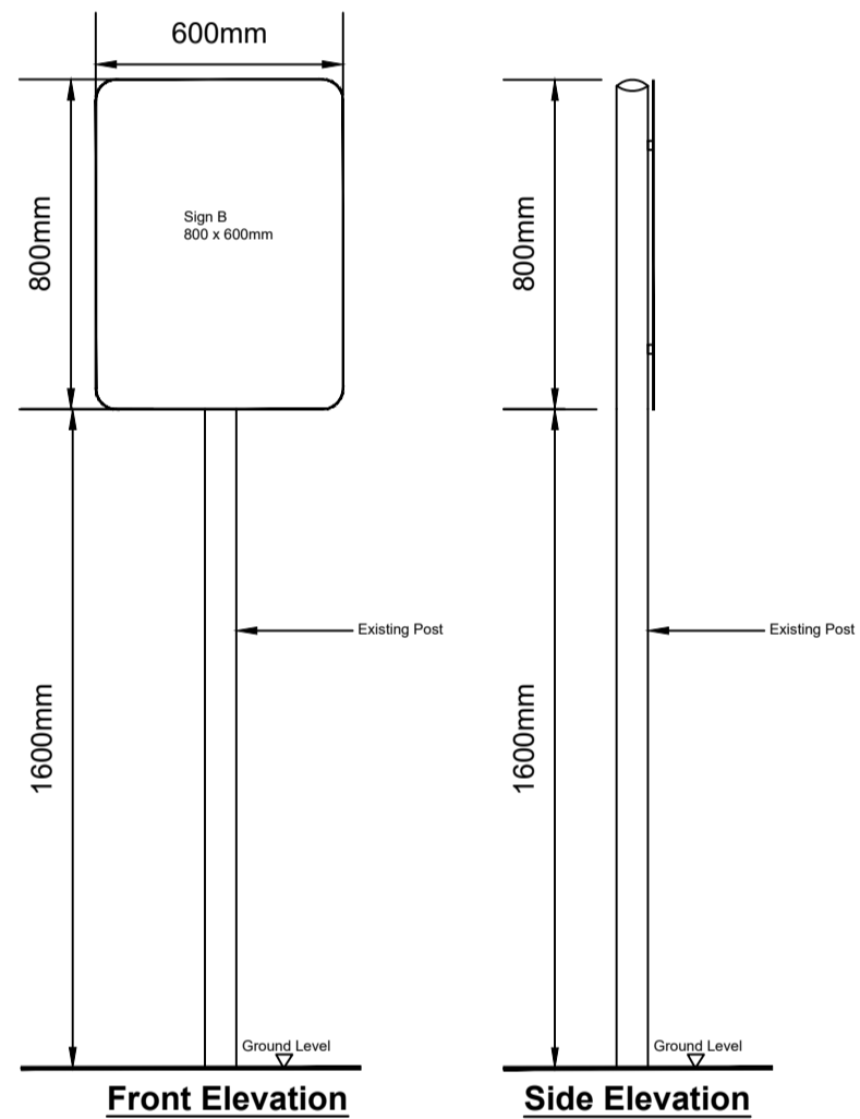
Sign #8 Mounted on old existing posts 1600mm from ground level
