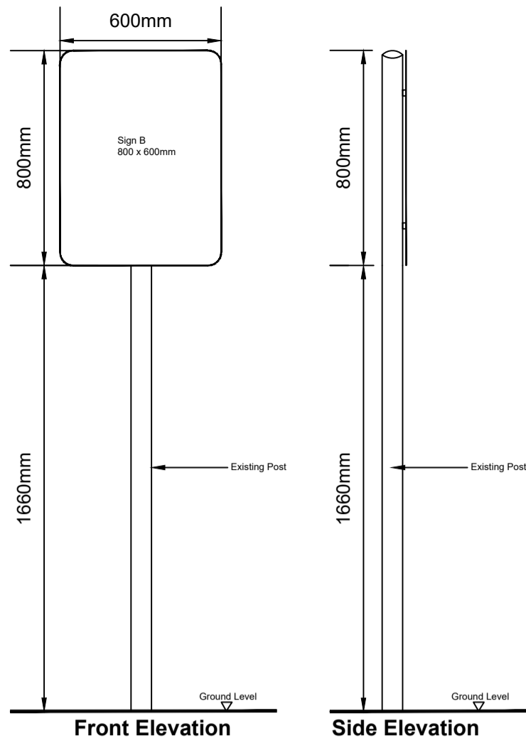
Sign #2 Mounted on old existing posts 1660mm from ground level
