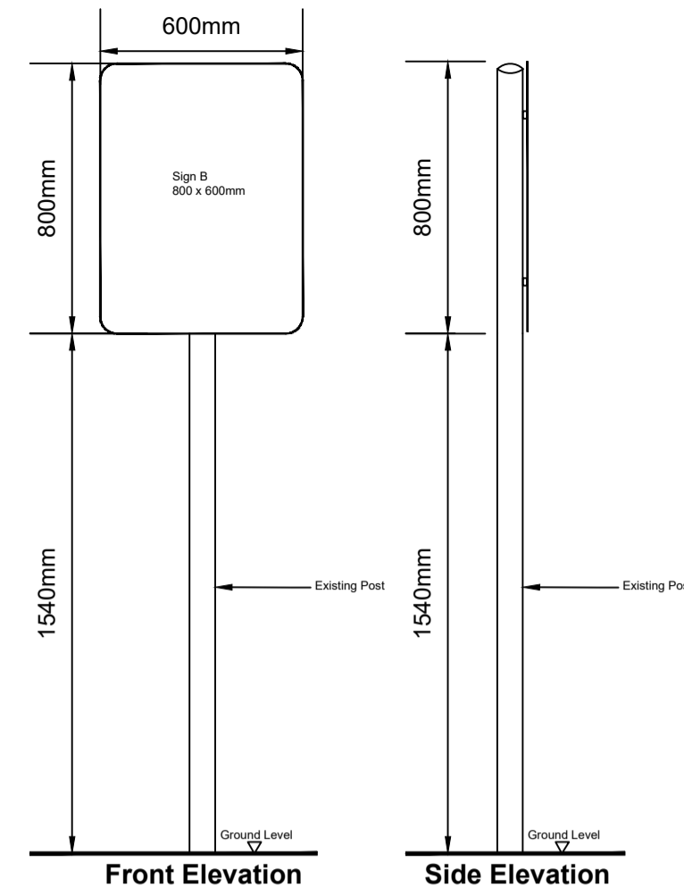
Sign #7 Mounted on old existing post 1540mm from ground level
