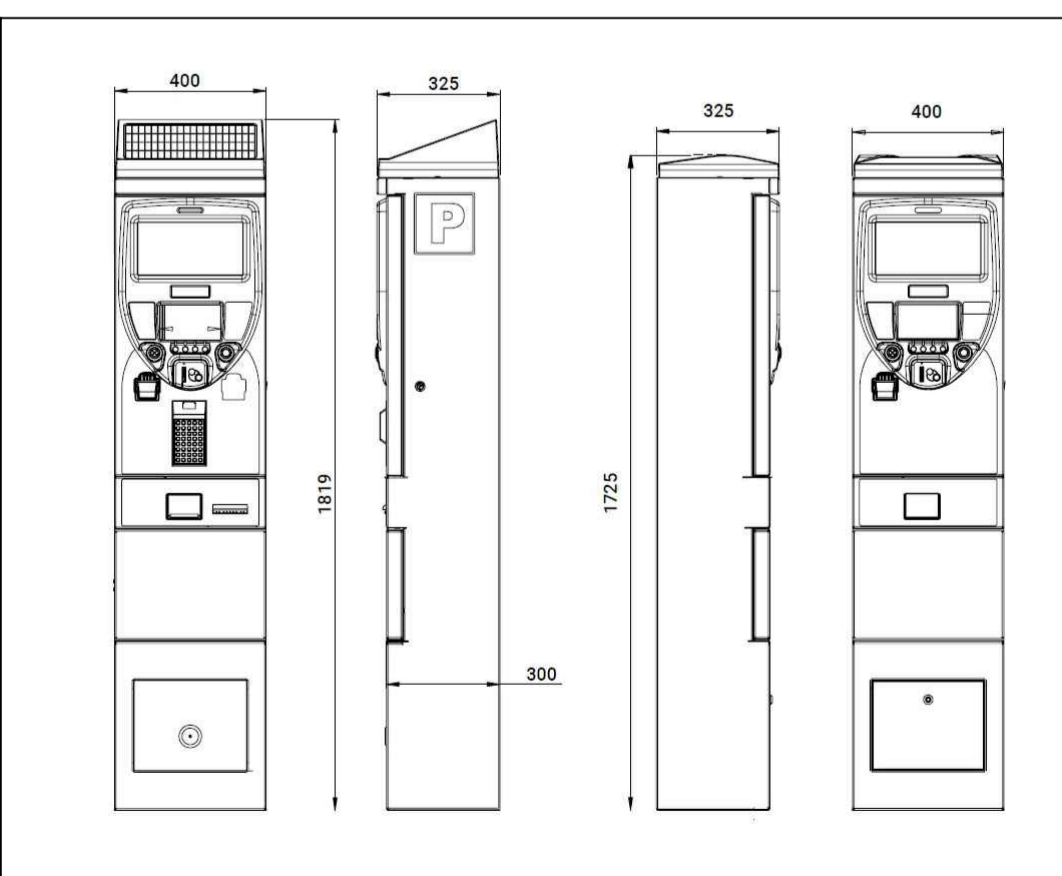
Pay Machine Scale 1:20
