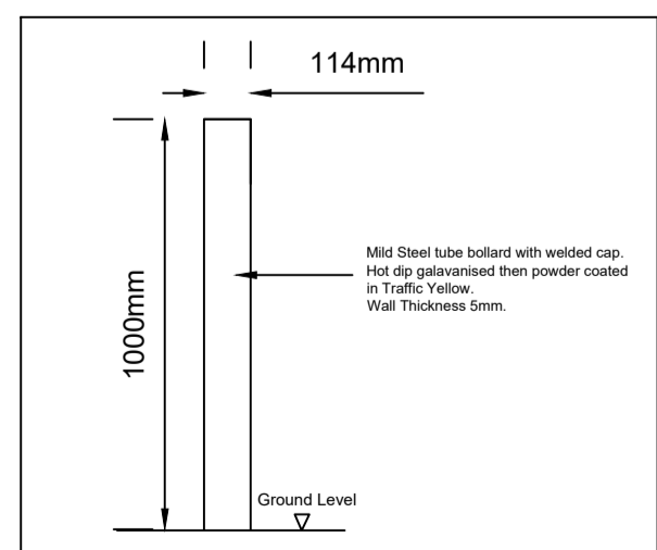
Bollard Scale 1:20
