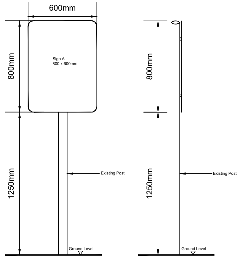
Sign #1 Mounted on old existing post 1250mm from ground level
