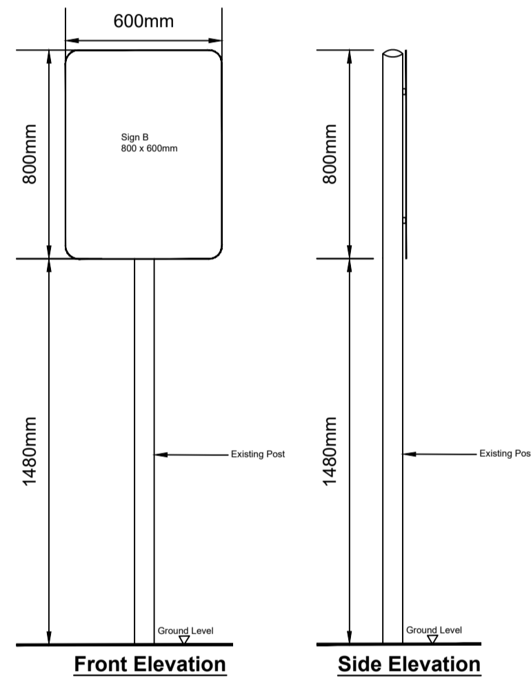
Sign #9 Mounted on old existing posts 1480mm from ground level
