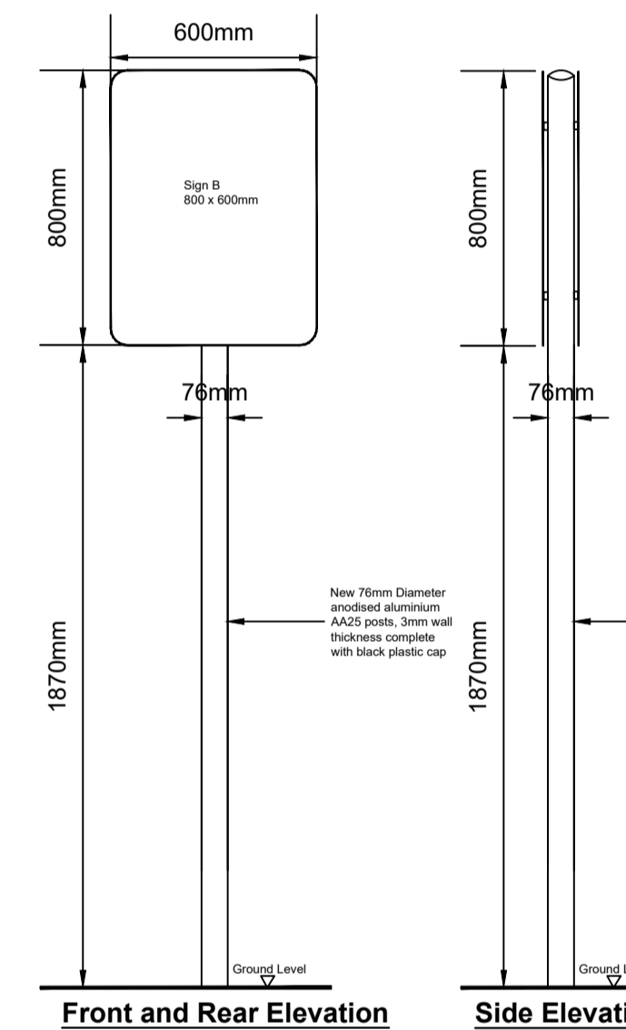
Sign #10 and #11 Double Sided Mounted on new posts 1870mm from ground level
