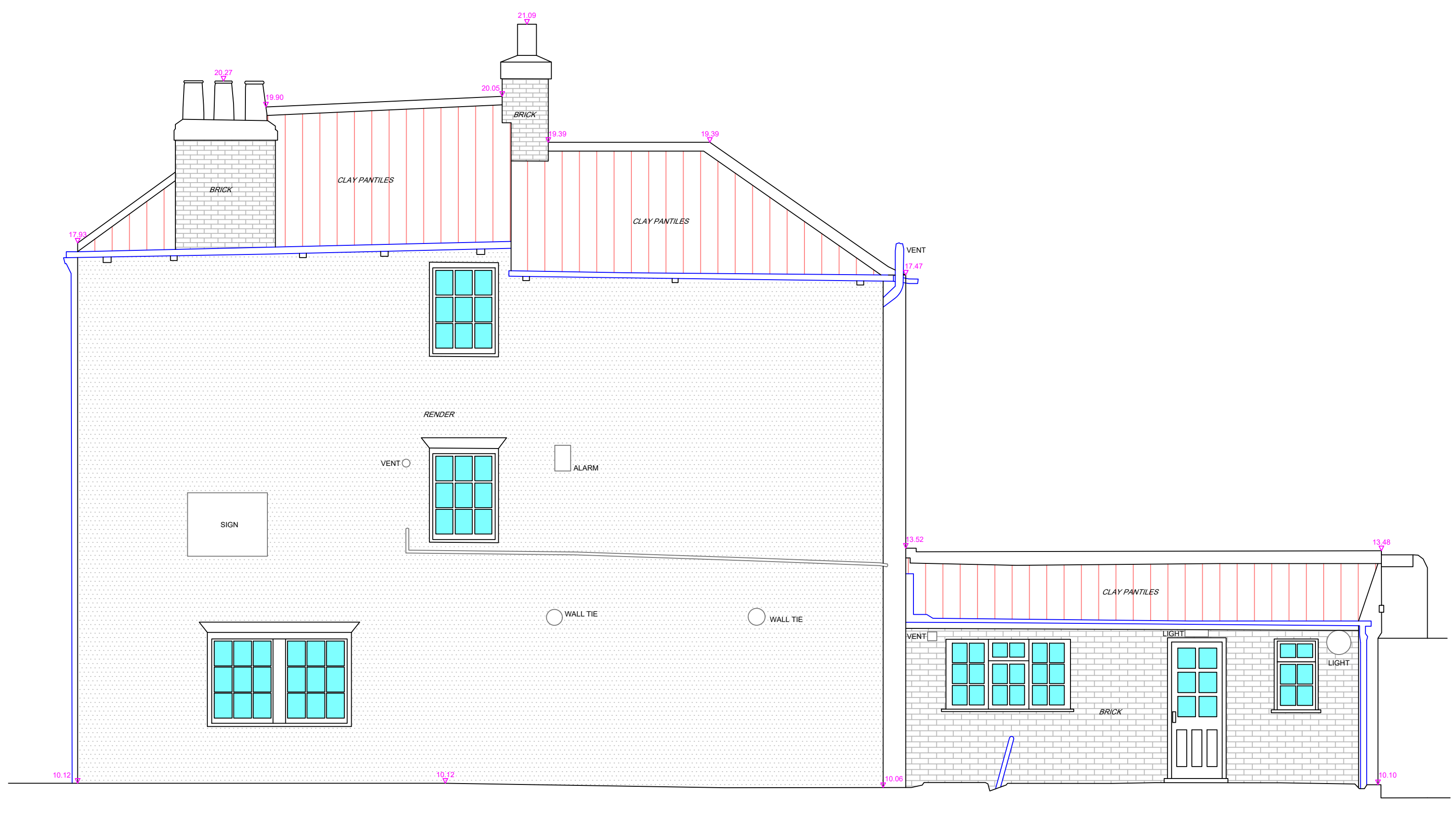
DATUM 8.20m A.O.D. ELEVATION 2
