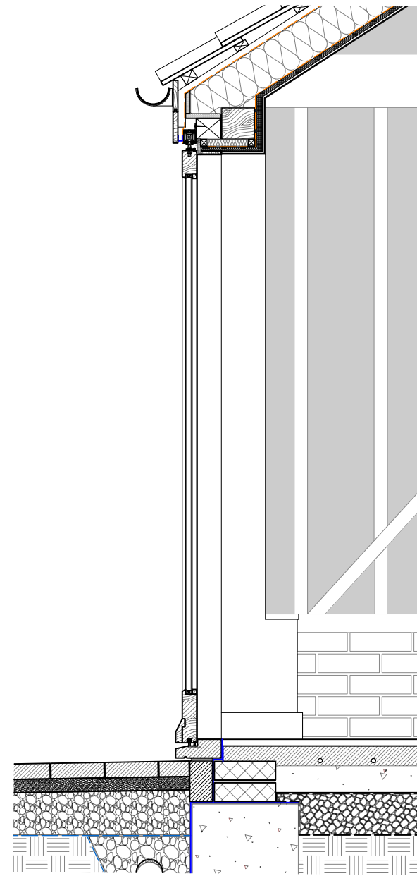
SECTION
