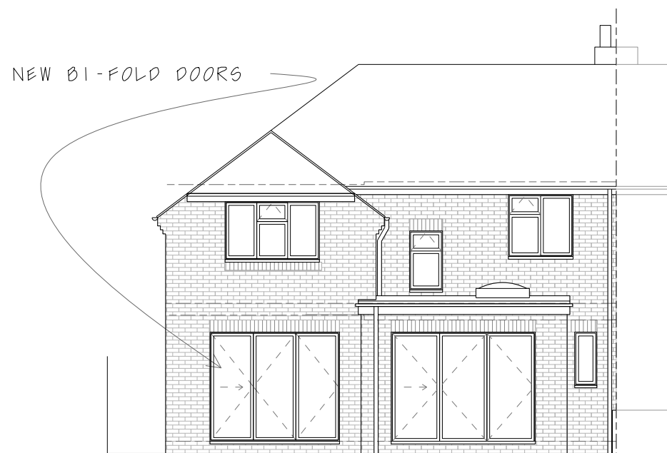
PROPOSED REAR ELEVATION (S)
