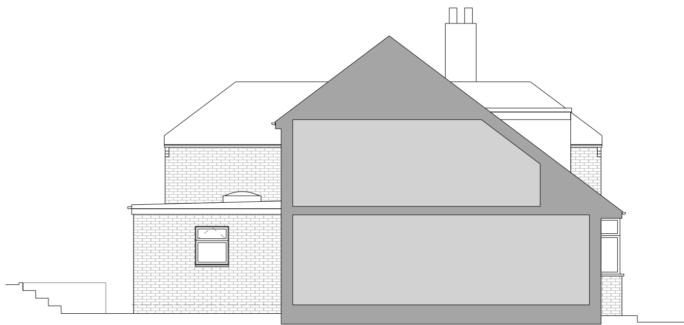
PROPOSED SIDE ELEVATION (E)
