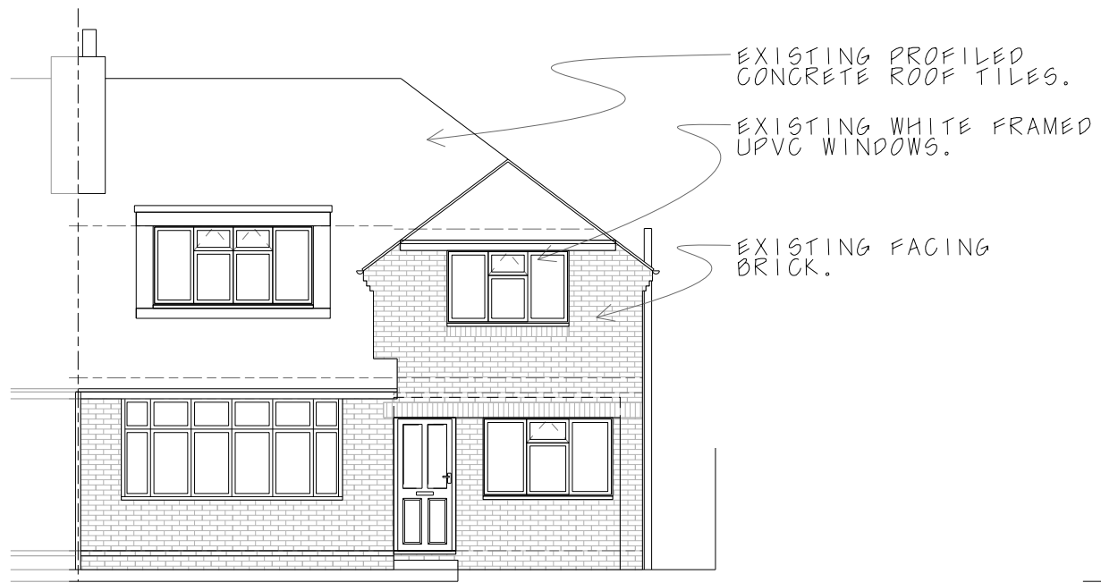
EXISTING FRONT ELEVATION (N)
