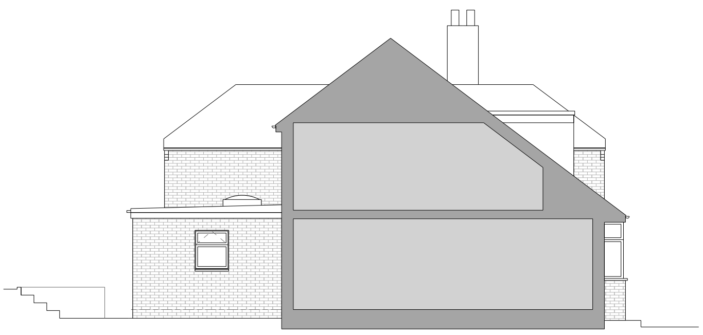
EXISTING SIDE ELEVATION (E)
