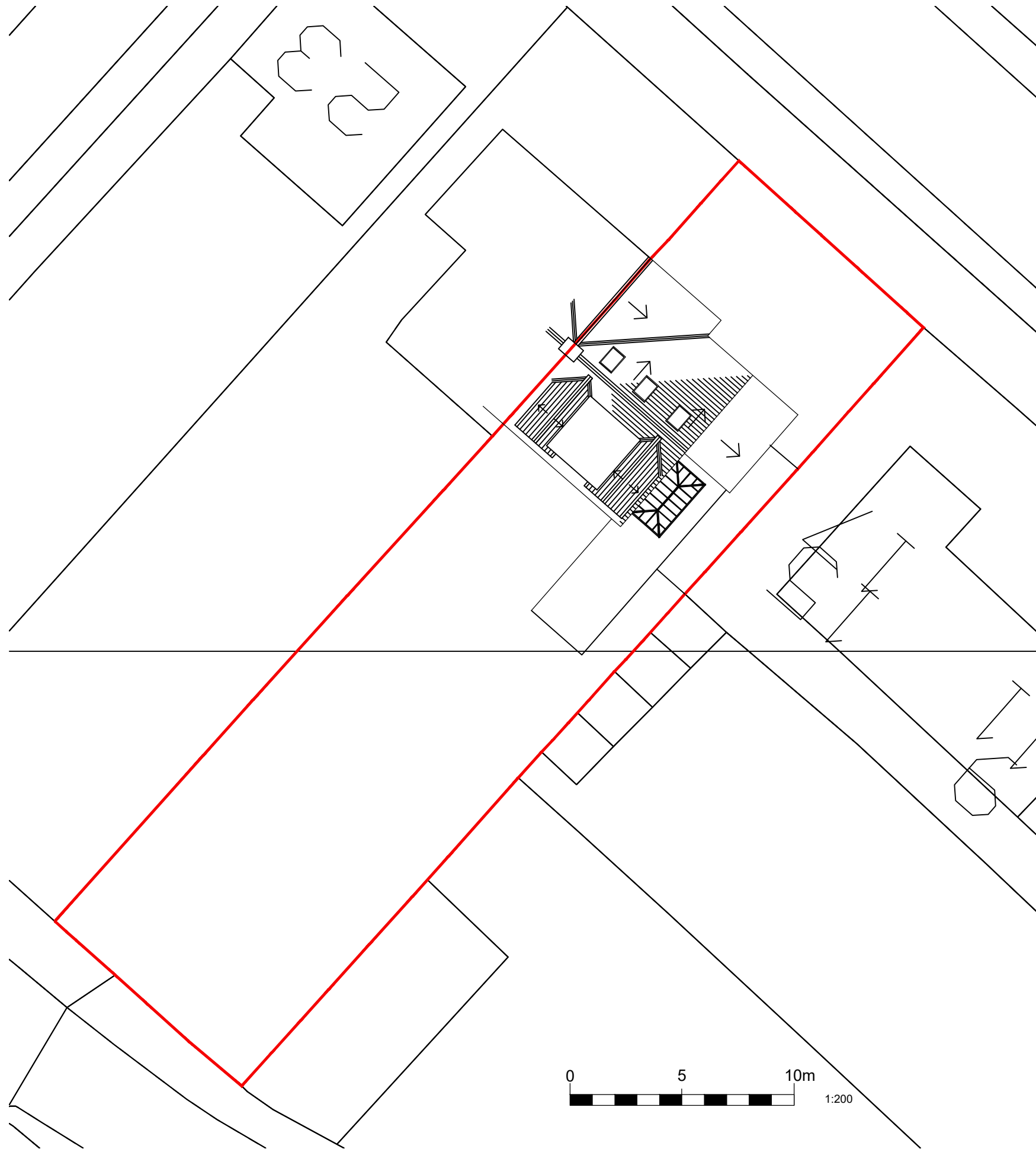
PROPOSED SITE PLAN (1:200 @ A3)
