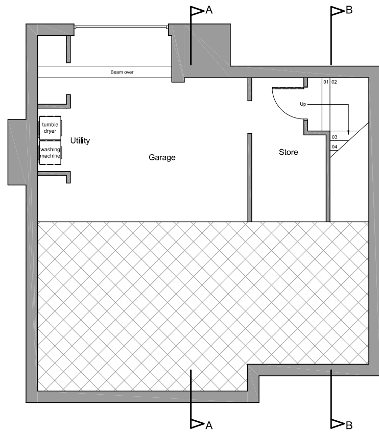
Basement plan
