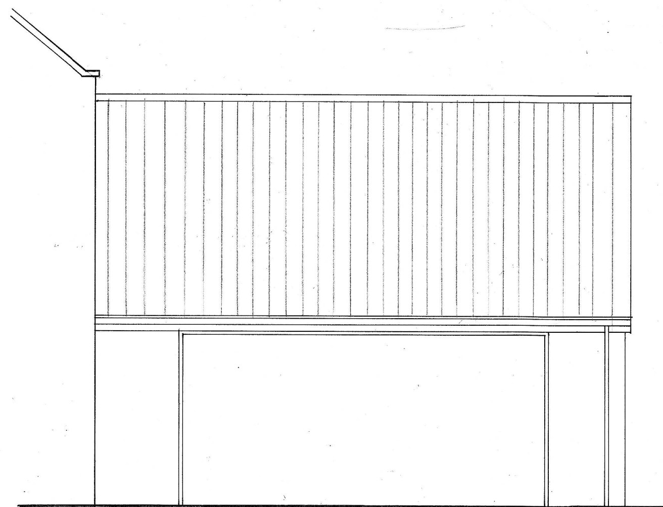
ELEVATION D
