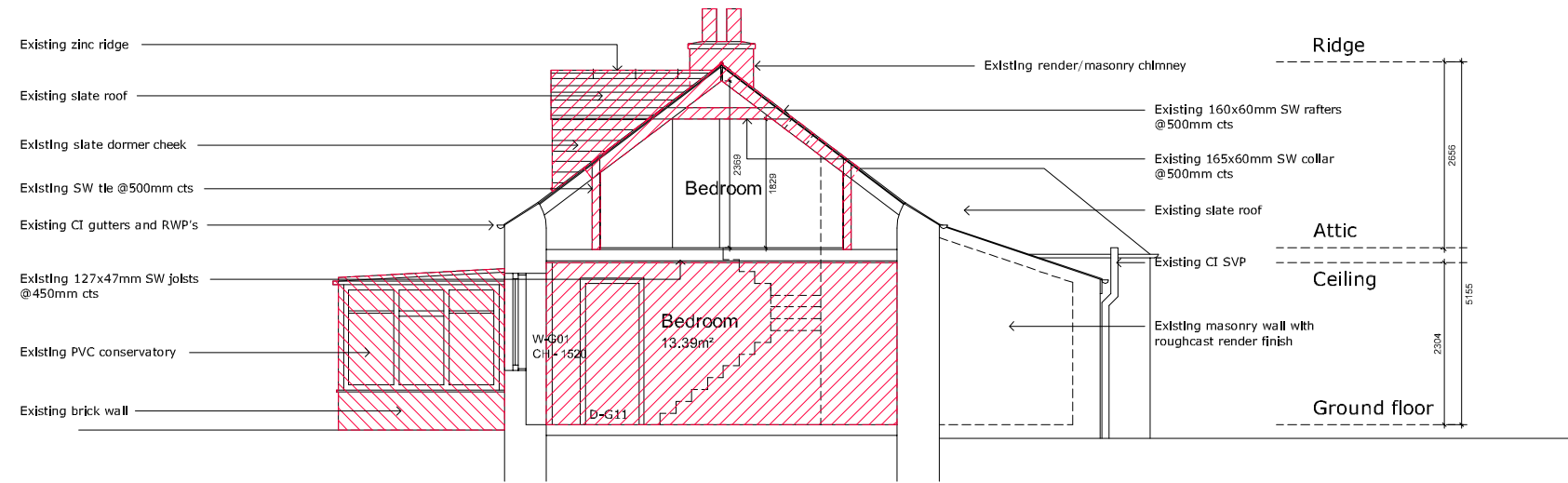
EXISTING SECTION C-C
