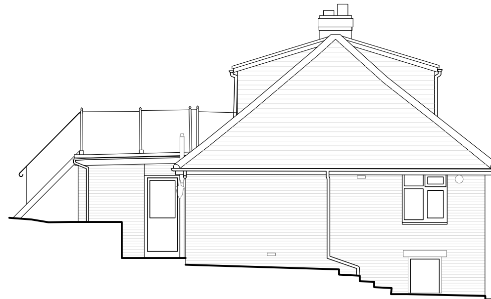
EAST ELEVATION
