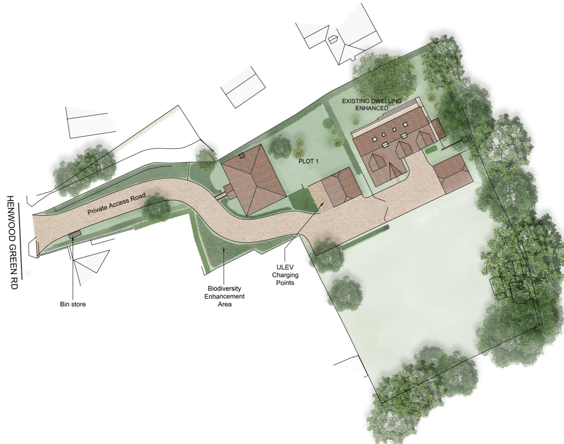
SITE PLAN
