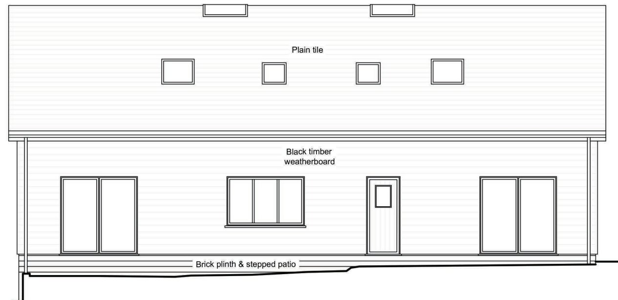
NORTH ELEVATION
