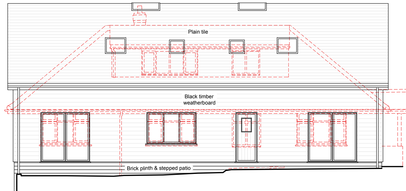
NORTH ELEVATION
