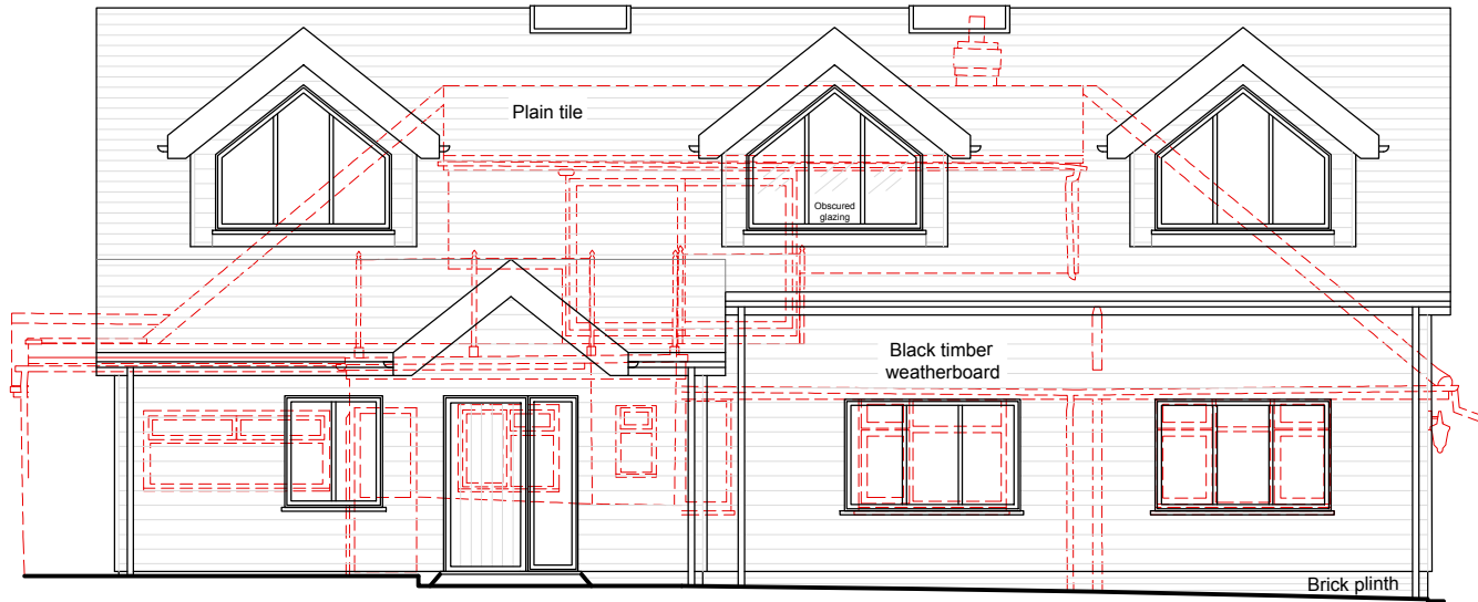
SOUTH ELEVATION
