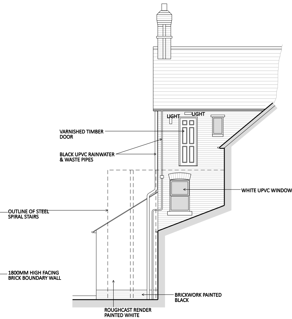
EXISTING REAR ELEVATION - C
