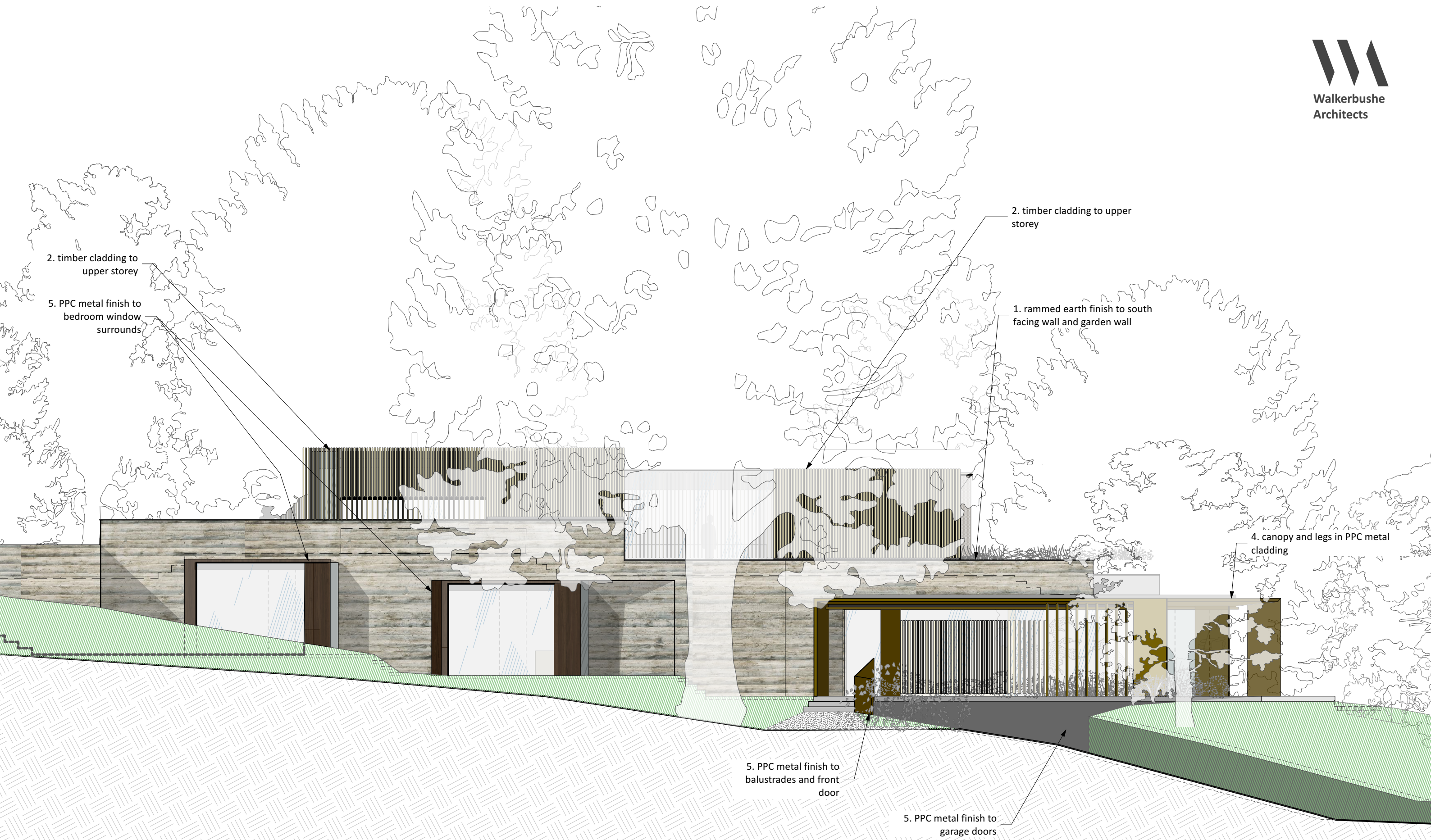
1 proposed south elevation- materials Scale: 1:100
