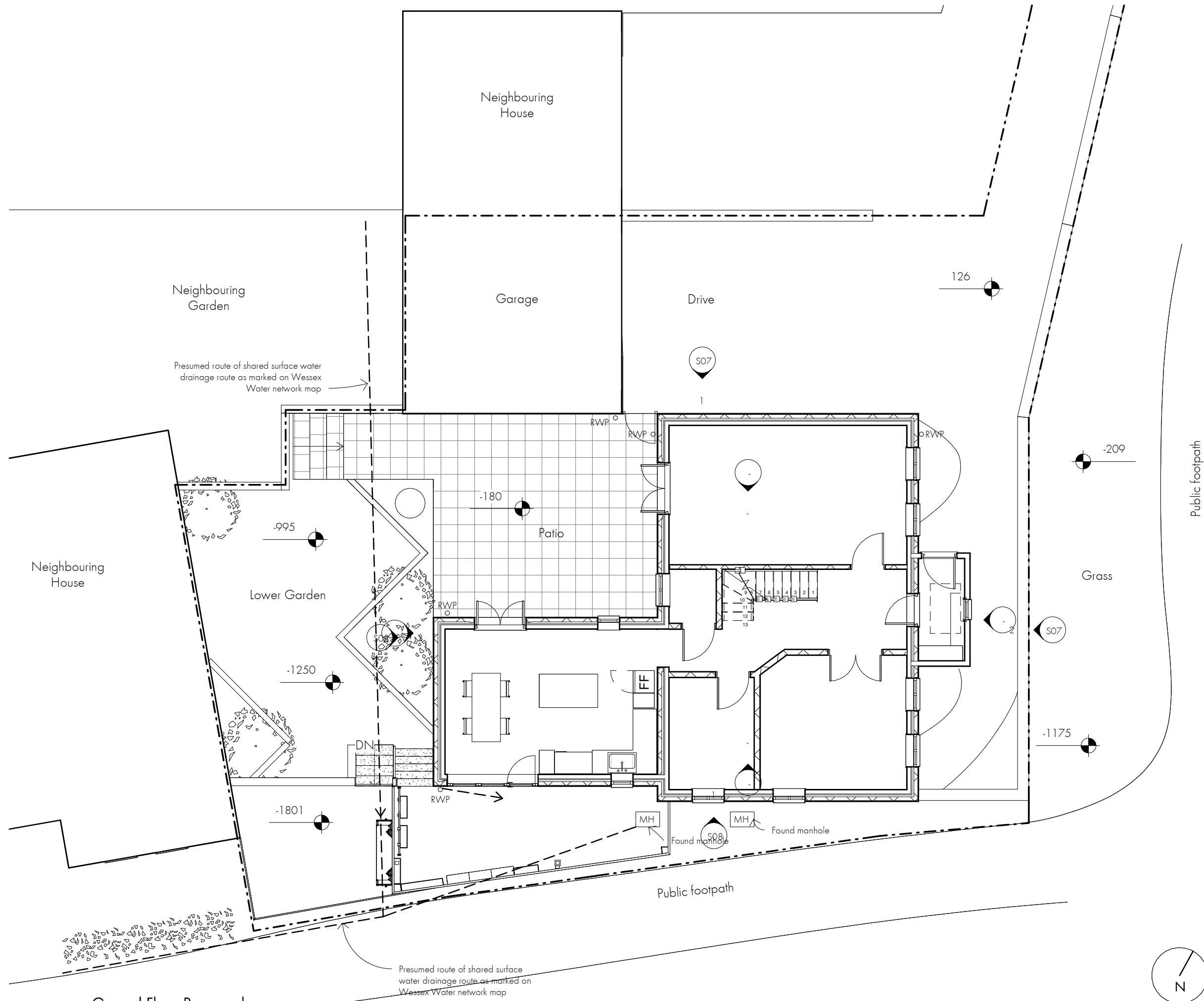
1 Ground Floor Proposed 1:100
